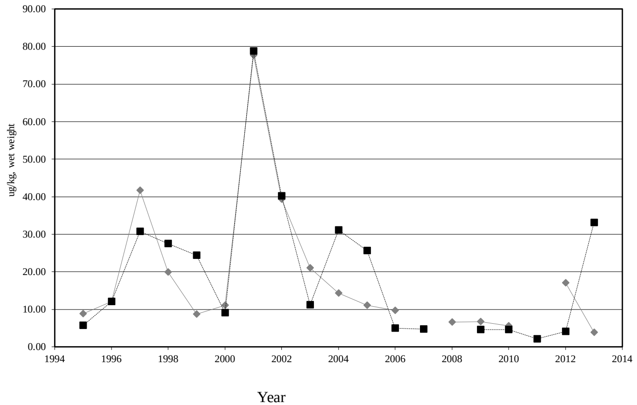
Figure A-36. Average total DDT concentrations (ug/kg) in rockfish muscle at 98 meter rig fishing (RF) stations during October (1995-2013).
