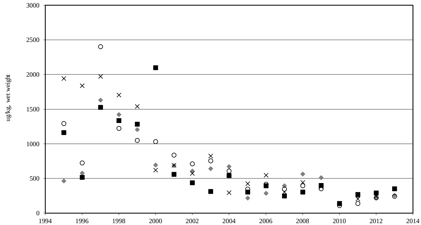
Figure A-30. Average total DDT concentrations (ug/kg) in flatfish liver at 98 meter trawl fishing zone (TFZ) stations during October (1995-2013).
