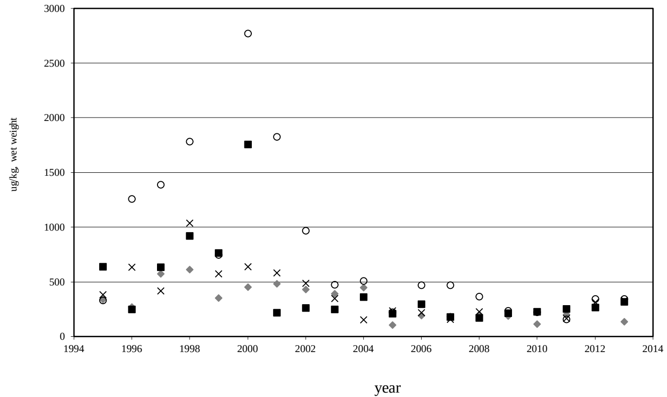
Figure A-31. Average total PCB concentrations (ug/kg) in flatfish liver at 98 meter trawl fishing zone (TFZ) stations during October (1995-2013).
