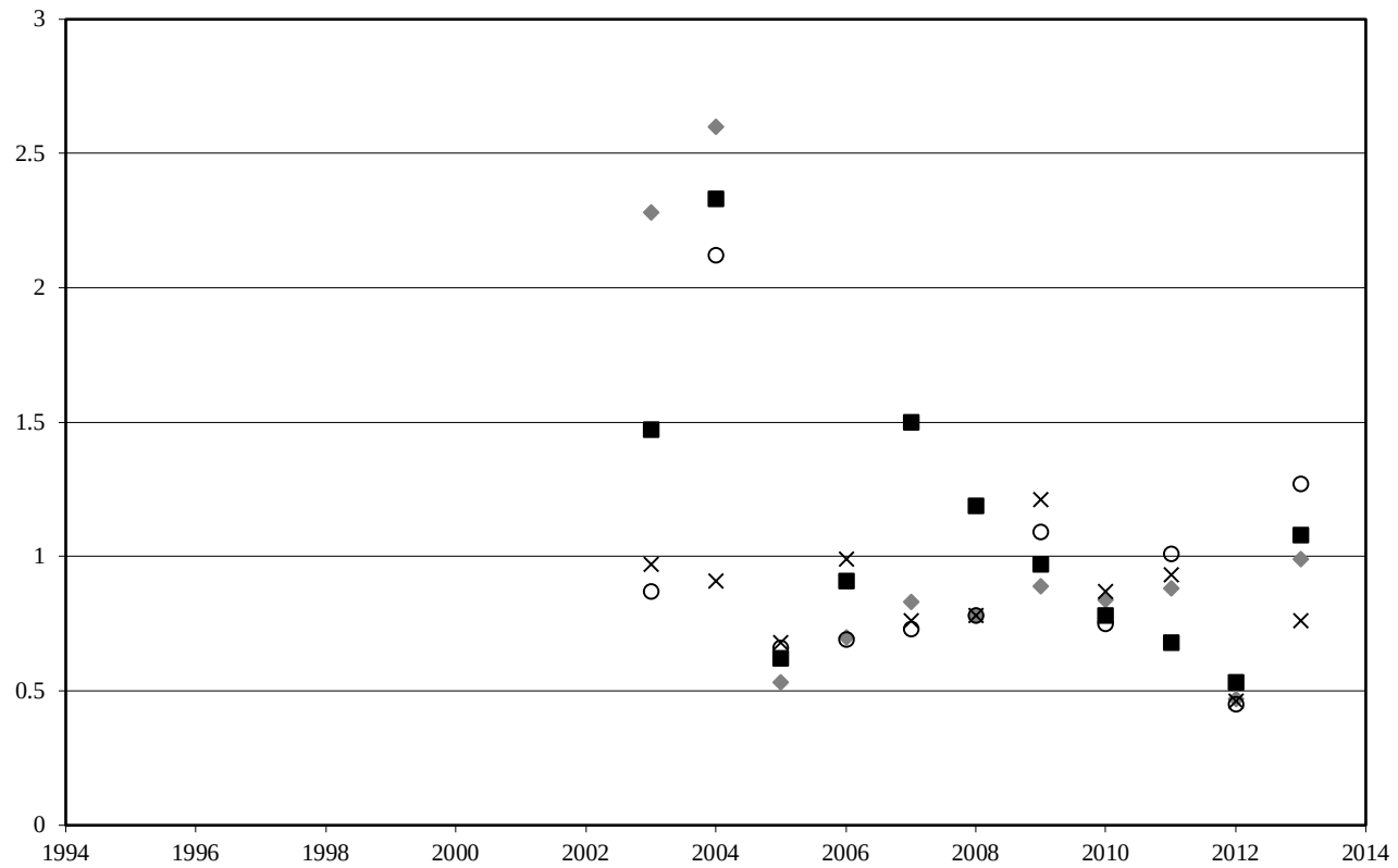
Figure A-27. Average selenium concentrations (mg/kg ww) in flatfish liver at trawl fishing zone stations during October (2003-2013).
