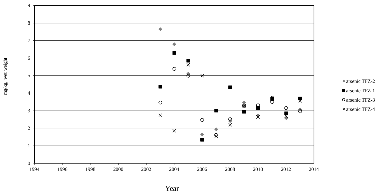
Figure A-25. Average total arsenic concentrations (mg/kg ww) in flatfish liver at 98 meter trawl fishing zone (TFZ) stations during October (2003-2013).
