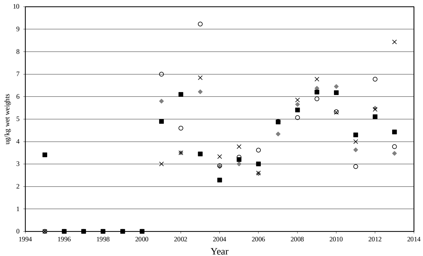
Figure A-28. Total BHC concentrations (ug/kg) in flatfish liver at trawl fishing zone stations during October (1995-2013).
