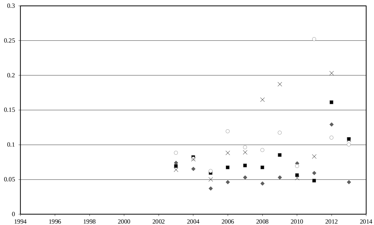
Figure A-26. Average mercury concentrations (mg/kg ww) in flatfish liver at trawl fishing zone stations during October (2003-2013).
