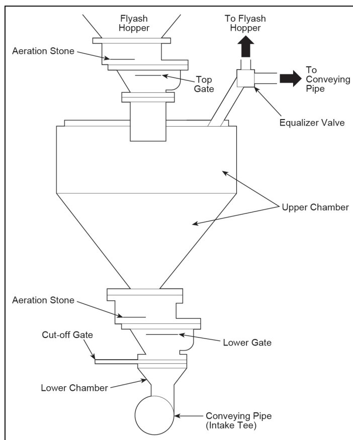
Figure 7-10. Pressure System Airlock Valve
