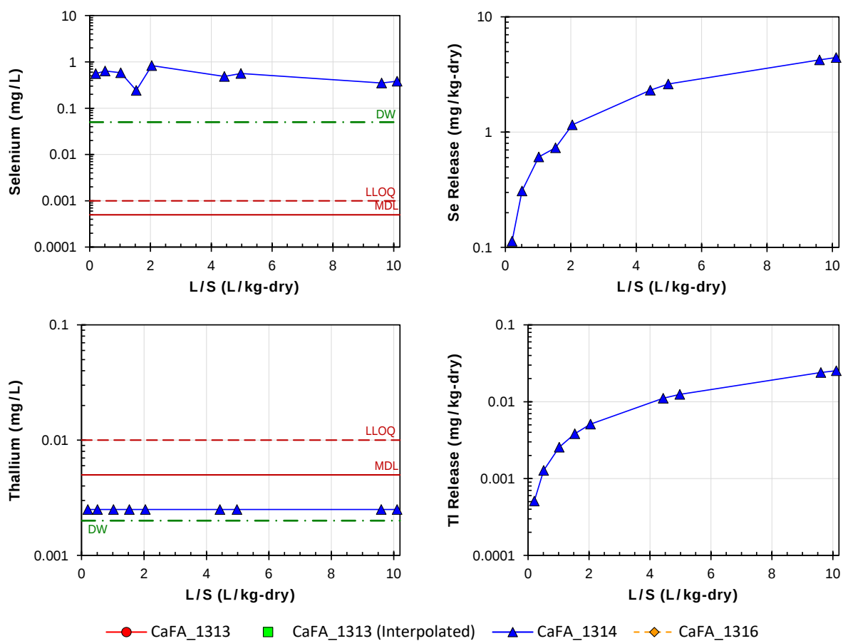
Figure B-16. Method 1314 results for a low-carbon coal fly ash (CaFA): Selenium and thallium.
