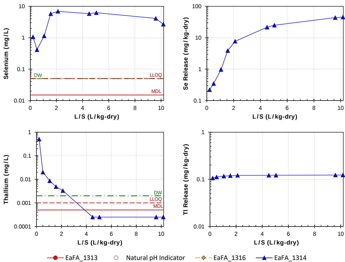
Figure B-6. Method 1314 results for a low-carbon coal fly ash (EaFA): Selenium and thallium.
