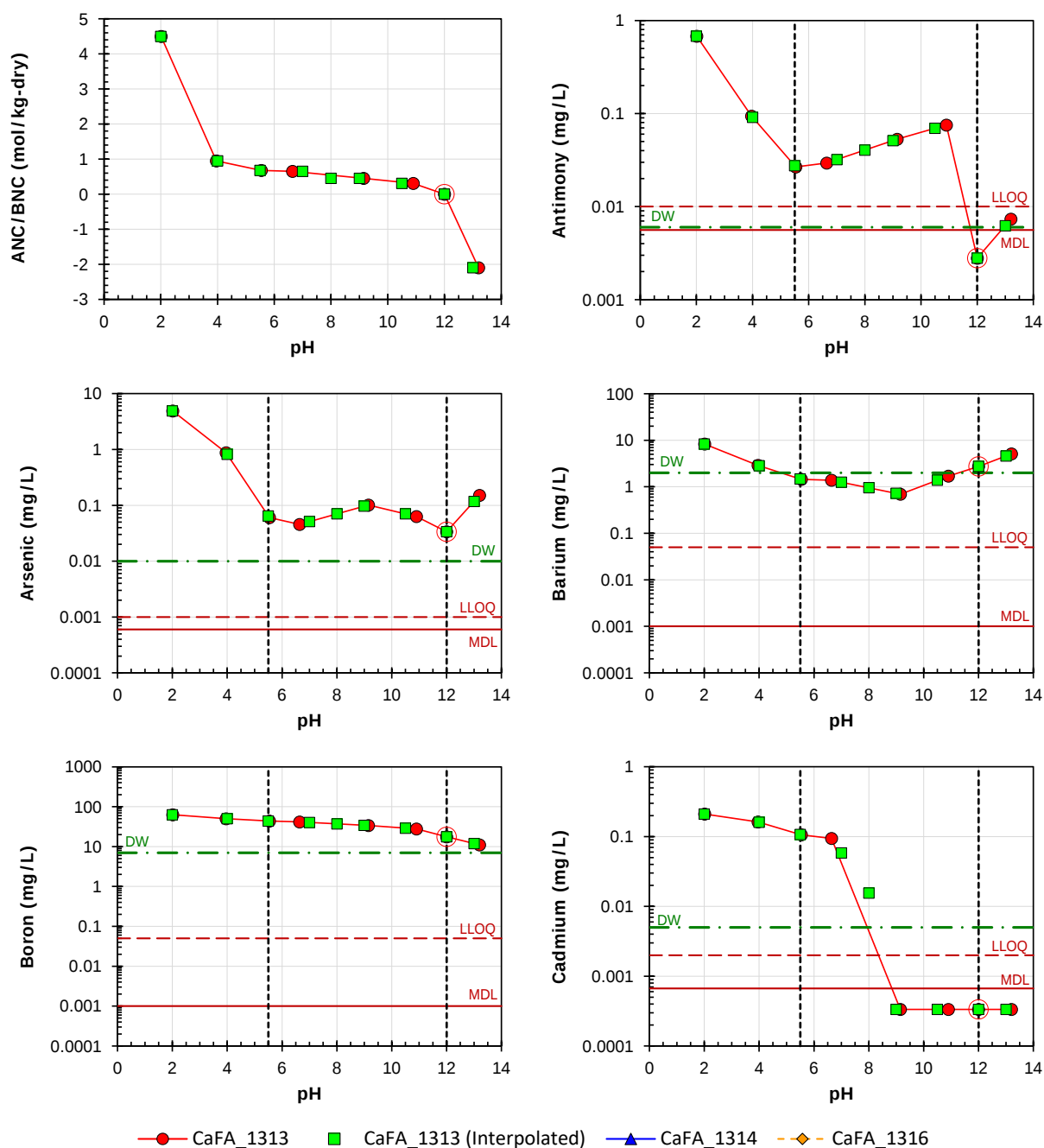
Figure B-11. Method 1313 results for a high-carbon coal fly ash (CaFA):
