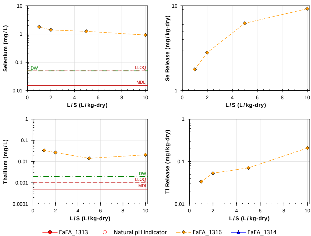
Figure B-10. Method 1316 results for a low-carbon coal fly ash (EaFA): Selenium and thallium.
