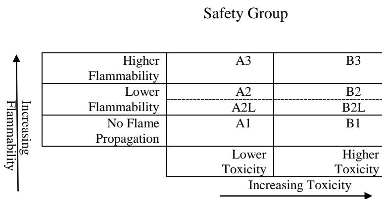
Figure 1. Refrigerant Safety Group Classification
