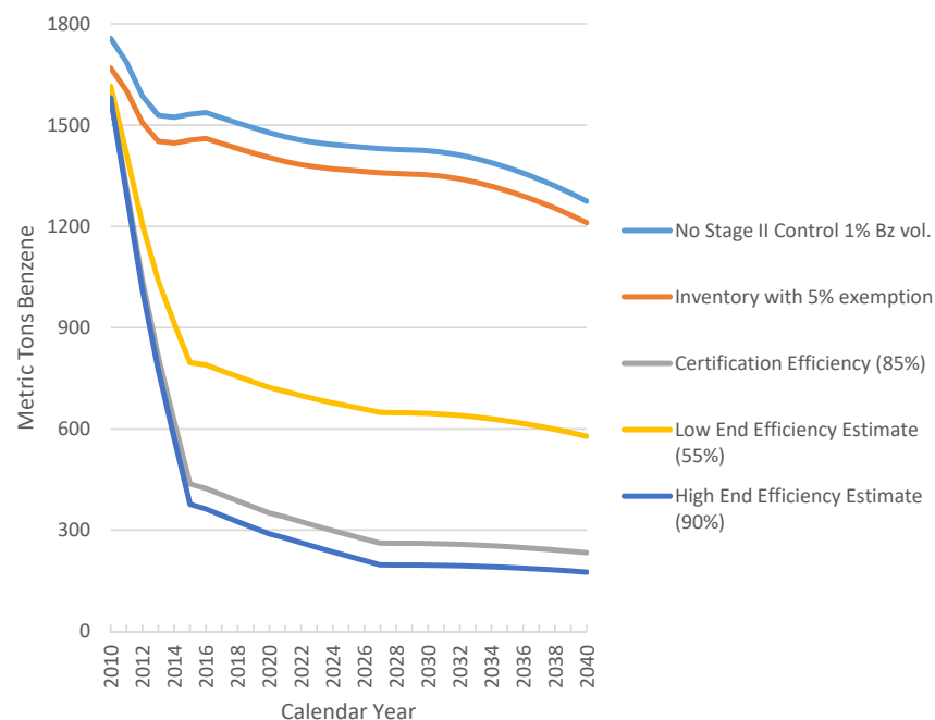
EU Refueling Benzene Emissions Inventory
