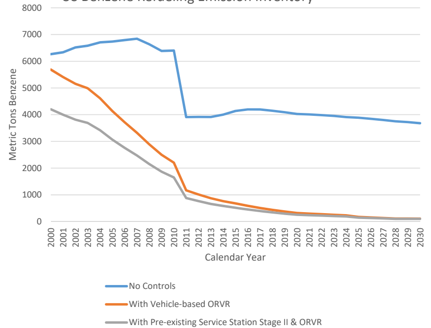
US Benzene Refueling Emission Inventory
