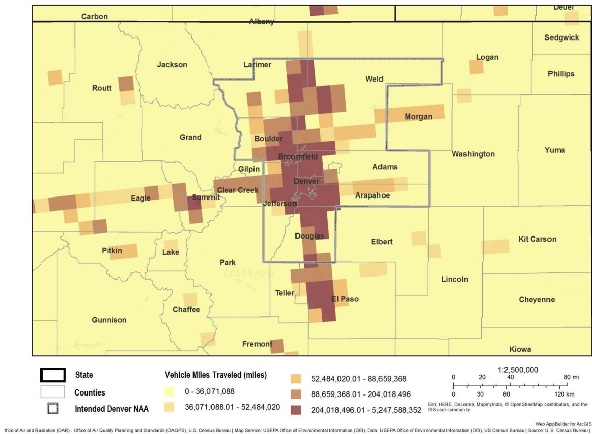
Figure 7. Twelve Kilometer Gridded VMT (Miles) Overlaid with Transportation Arteries.
