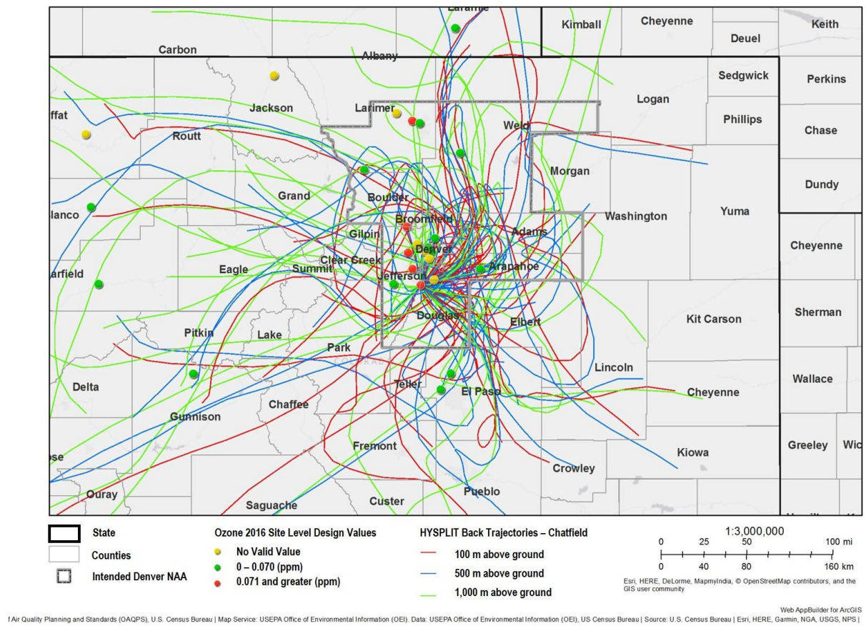
Figure 11. HYSPLIT Back Trajectories for Chatfield (Violating Monitor).
