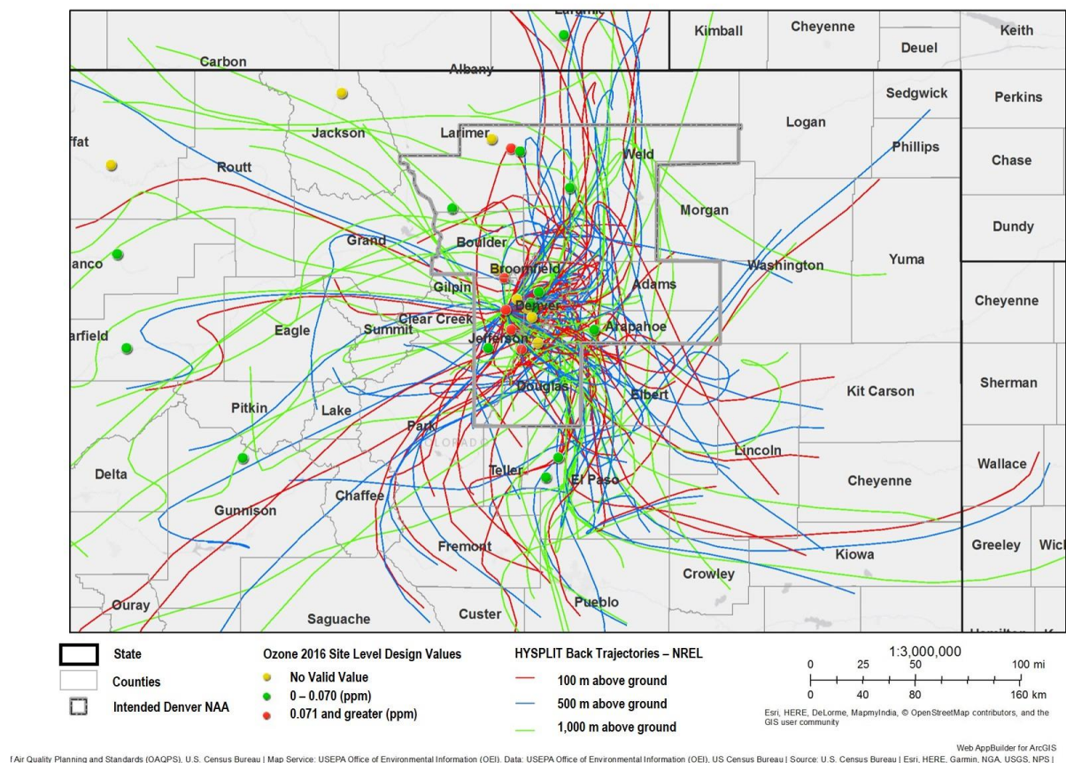
Figure 9. HYSPLIT Back Trajectories for NREL (Violating Monitor).
