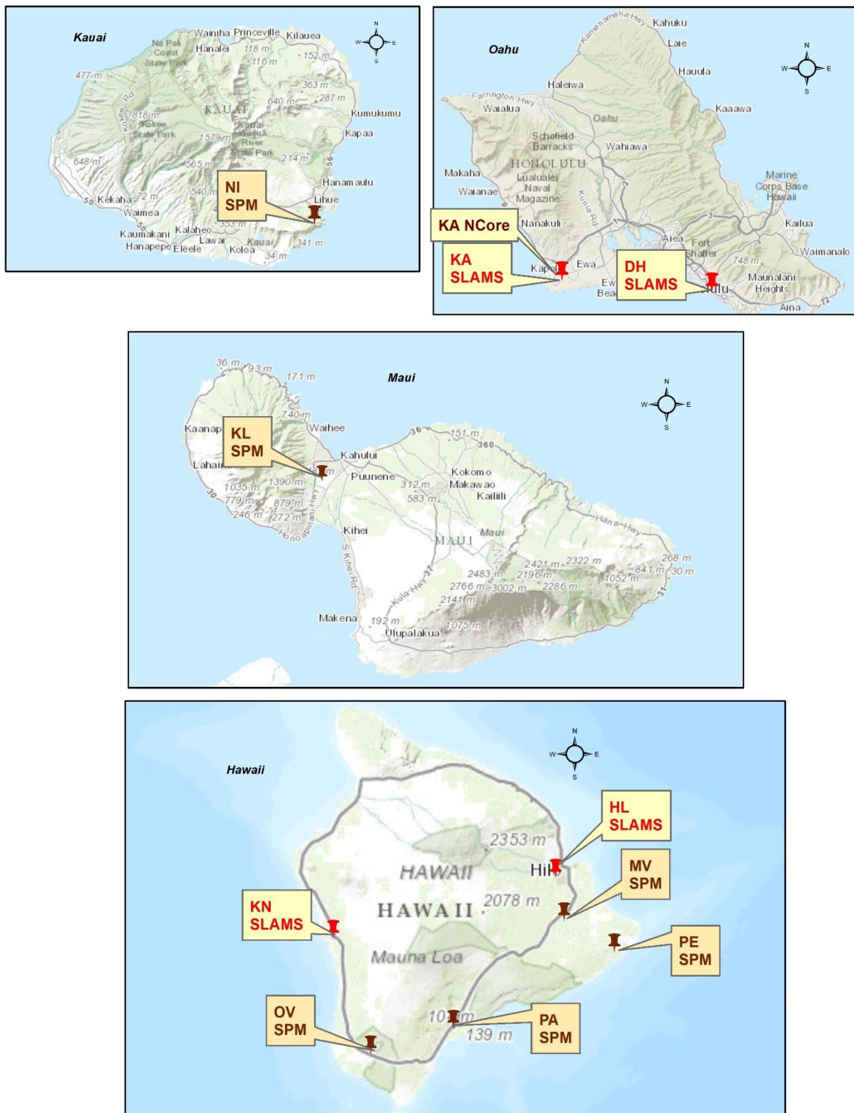
Figure 2-7. SO 2 Network
