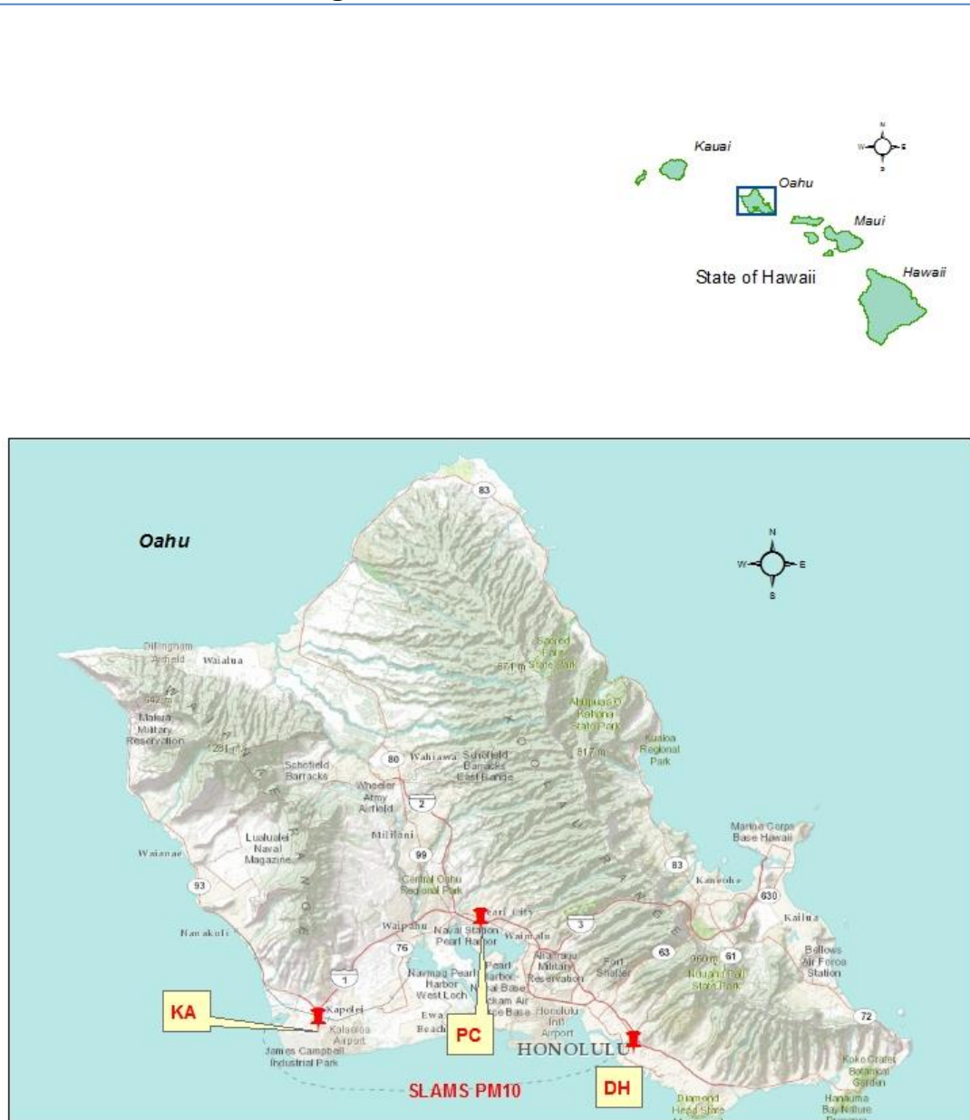
Figure 2-1. PM 10 Network
