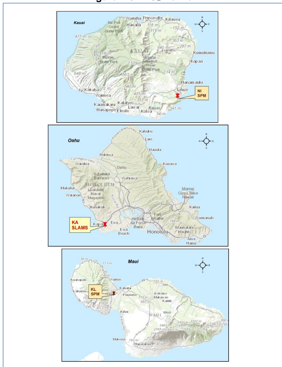
Figure 2-6. NO 2 Network
