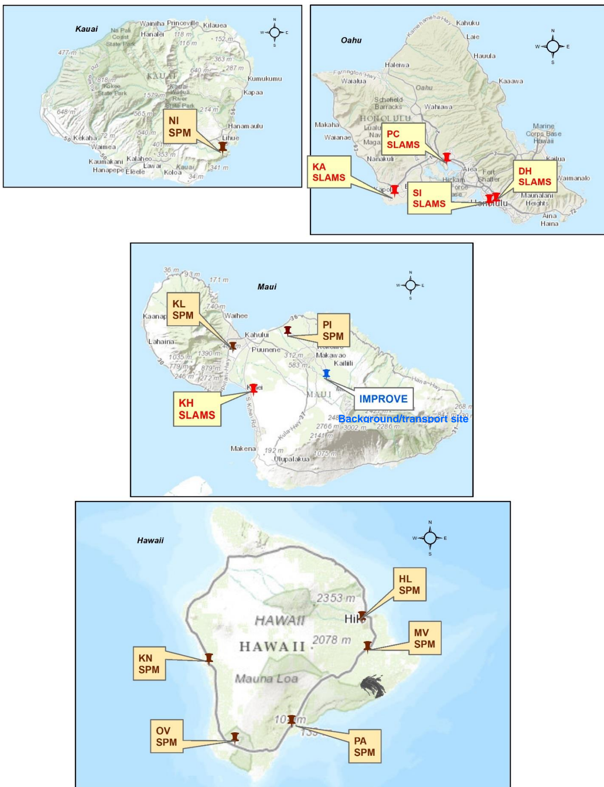
Figure 2-2. PM 2.5 Network
