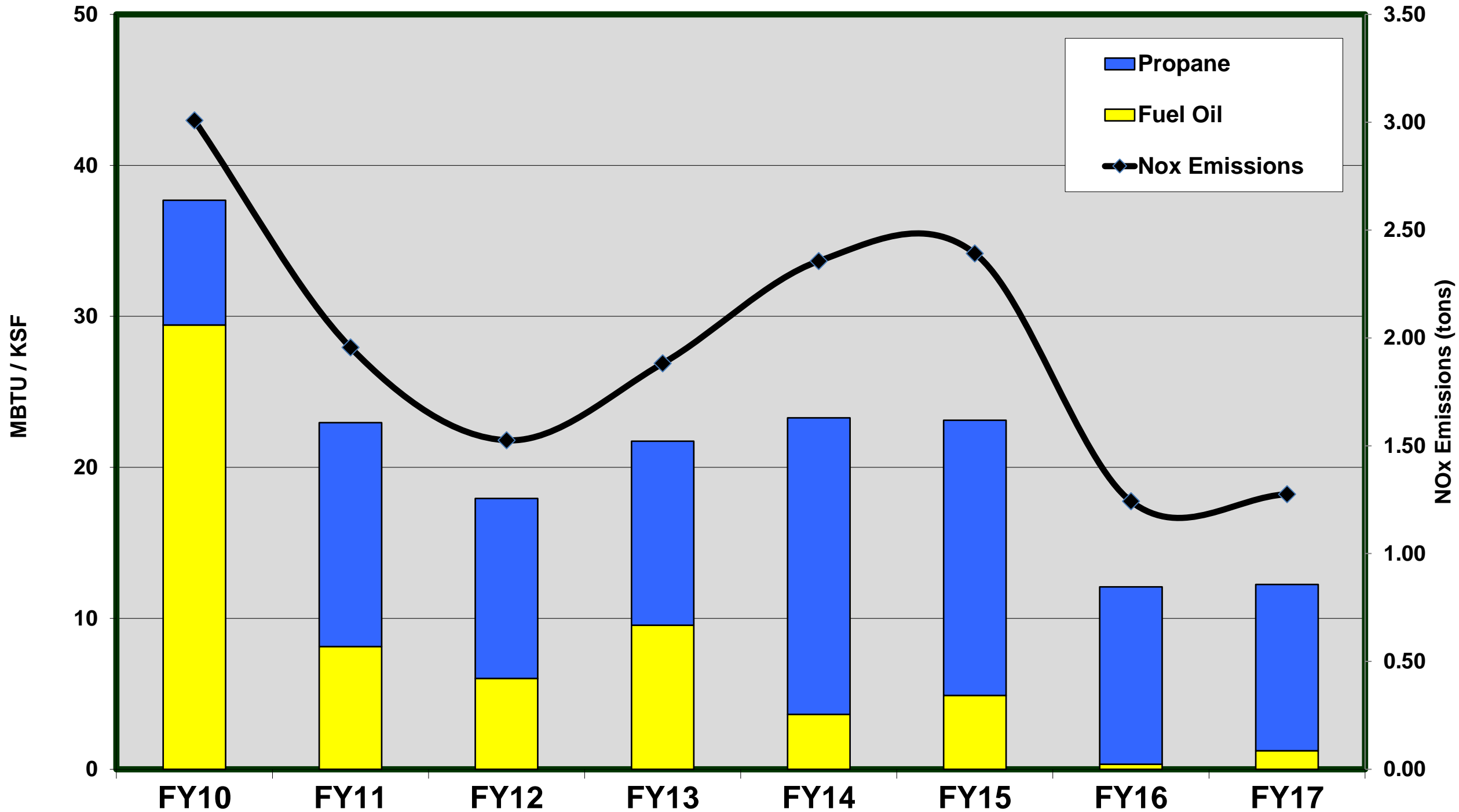
Fuel Use (MBTU/KSF) v. NOx Emissions (FY10 - FY16)
