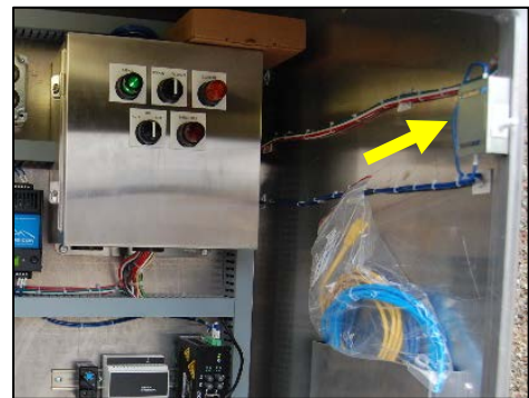
Figure 3-5. Door Alarm Switch
