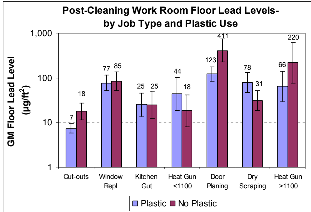
Figure 6-3. Post-Cleaning Work Room Floor Lead Levels, By Job and Plastic Use. The error bars represent the 95% confidence interval computed using the geometric standard deviation. The values presented on the graph are the geometric mean floor lead levels.
