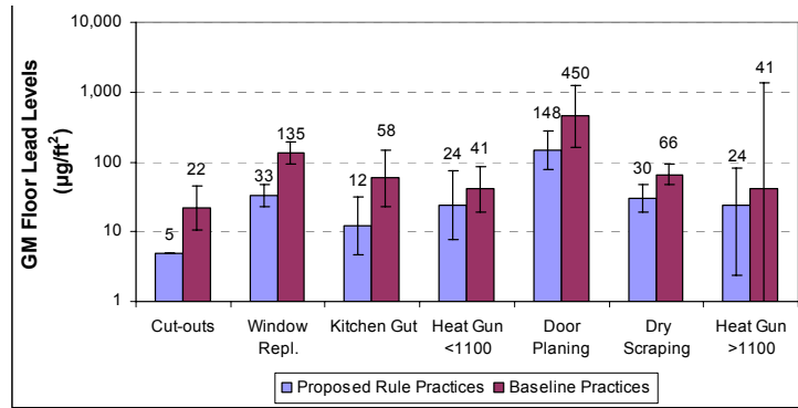
Figure 9-1. Post-Job Work Room Floor Lead Levels, By Job and Rule Use
