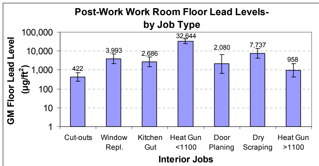
Figure 6-2. Post-work Floor Lead Levels in the Work Room, by Job Type. The error bars represent the 95% confidence interval computed using the geometric standard deviation. The values presented on the graph are the geometric mean floor lead levels.
