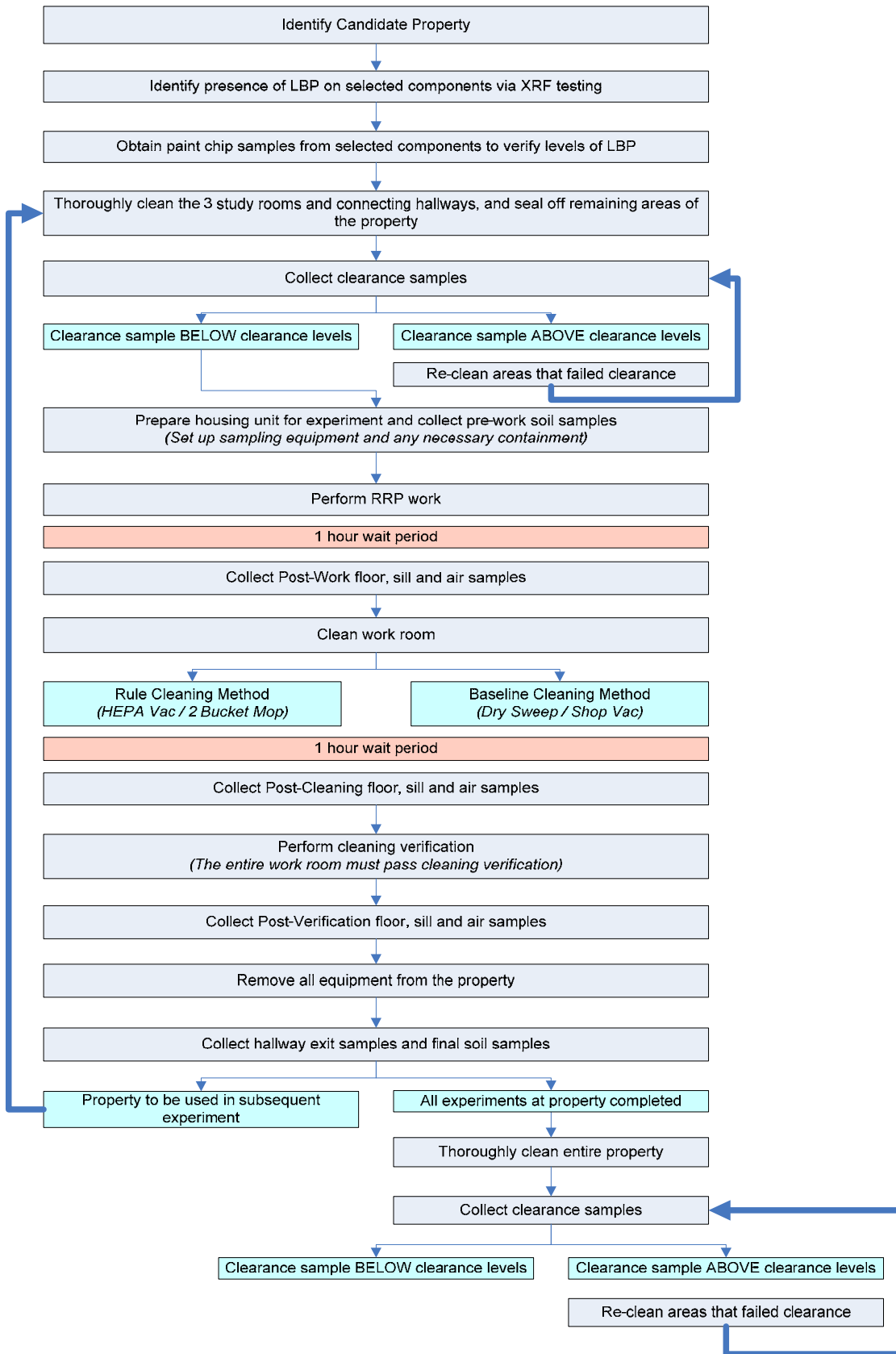
Figure 3-1. Flowchart of Interior Field Sampling Activities
