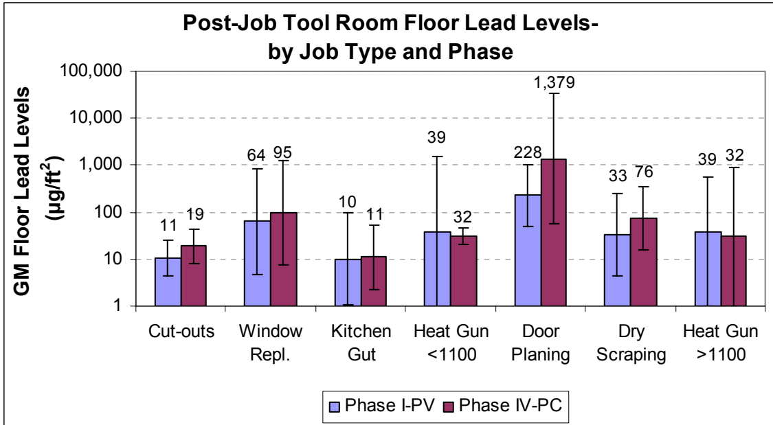
Figure 6-6. Post-Job Tool Room Floor Lead Levels, By Job and Phase. The error bars represent the 95% confidence interval computed using the geometric standard deviation. The values presented on the graph are the geometric mean floor lead levels.
