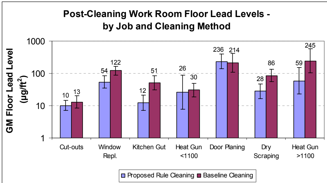
Figure 6-4. Post-Cleaning Work Room Floor Lead Levels, By Job and Cleaning Method. The error bars represent the 95% confidence interval computed using the geometric standard deviation. The values presented on the graph are the geometric mean floor lead levels.
