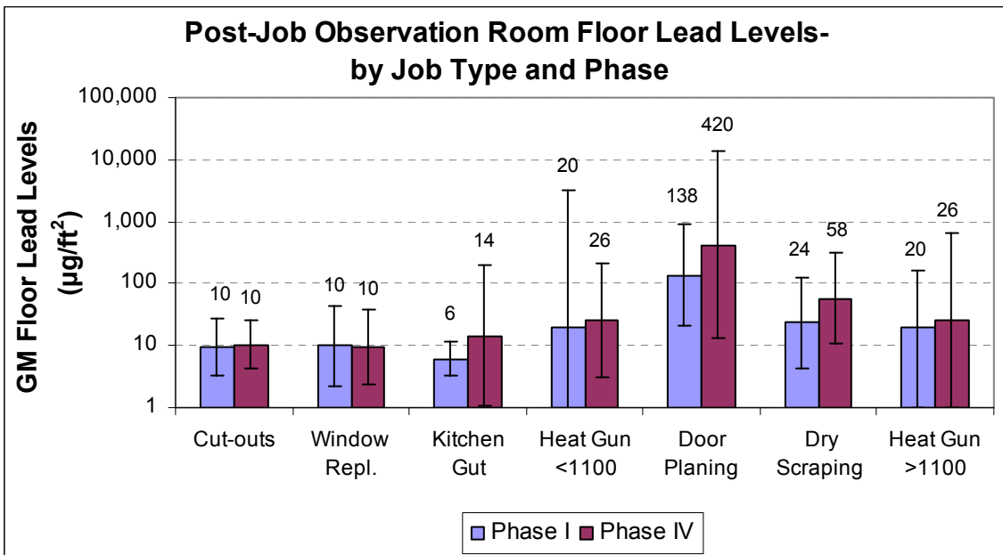
Figure 6-7. Post-Job Observation Room Floor Lead Levels, By Job and Phase. The error bars represent the 95% confidence interval computed using the geometric standard deviation. The values presented on the graph are the geometric mean floor lead levels.
