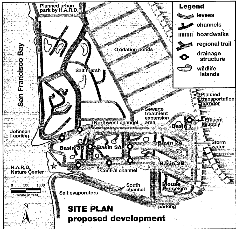
Schematic of the Hayward Shoreline Marsh Expansion Project.
