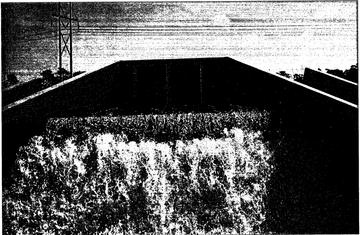
Figure 2. The influent structure aerates the water as it enters the wetland.
