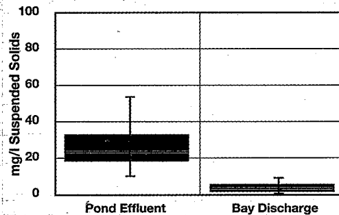
Pond and Wetland Suspended Solids Values
