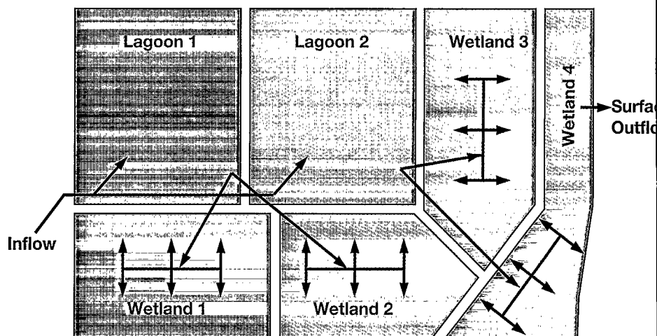
Figure 1. Layout of the Vermontville wastewater treatment system. Inflow may be directed to either of the two lagoons. The lagoons are discharged into wetlands 1-3. Wetland 4 no longer receives a direct discharge; but seepage water from the uphill units re-emerges into wetland 4.
