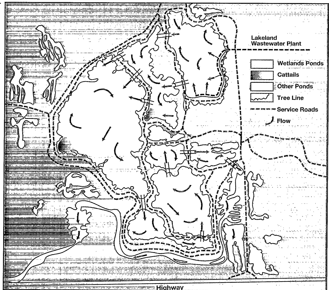
Figure 1. Plan view of the site showing the relative locations of the internal cells.
