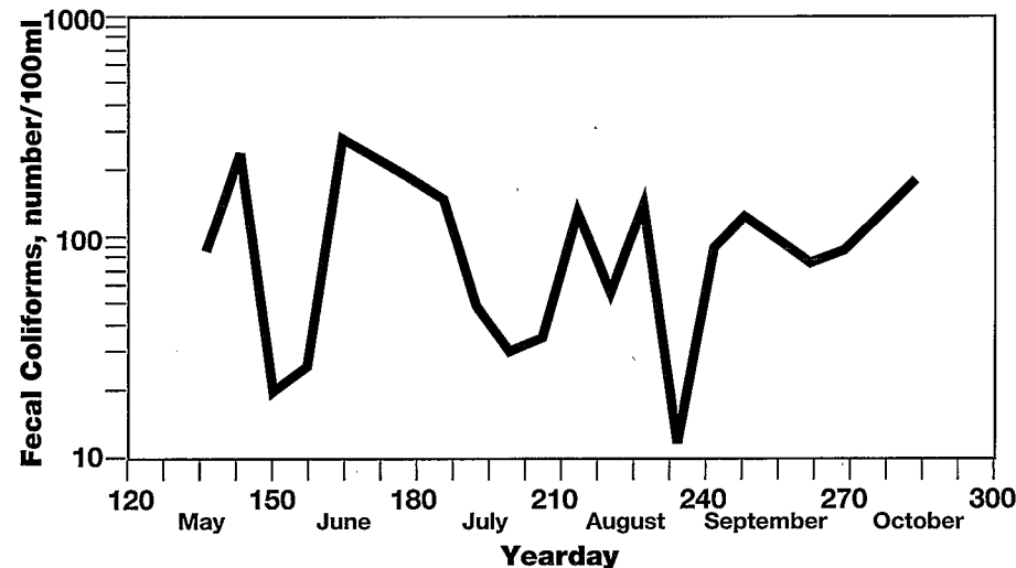
Figure 5. Fecal coliform bacteria counts also fluctuate in the outflow from the wetlands, but the seasonal average is quite low; the geometric mean value was 77. (Data are for 1990)
