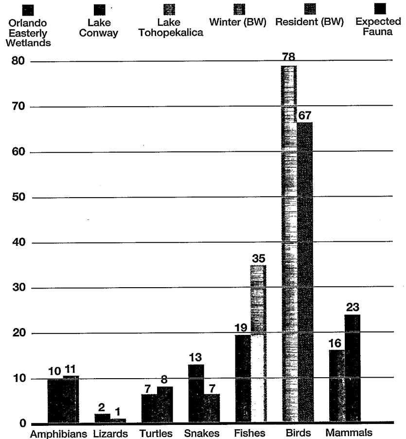
Figure 3 Comparison of Wildlife Diversity
