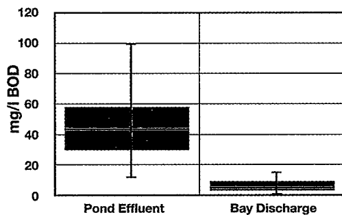
Pond and Wetland BOD Values
