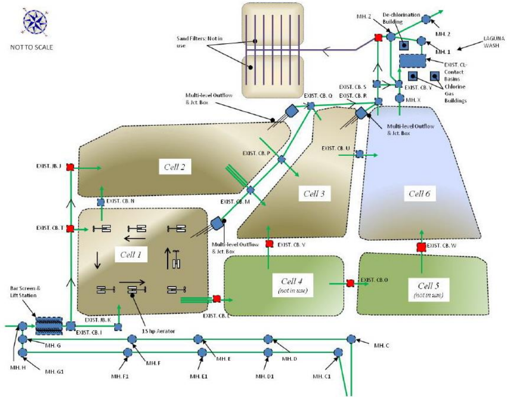
FIGURE 7: Existing Plant (As Currently Operated)
