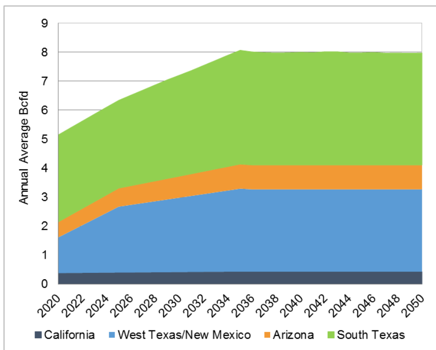
Figure 8-10 U.S. Pipeline Exports to Mexico
