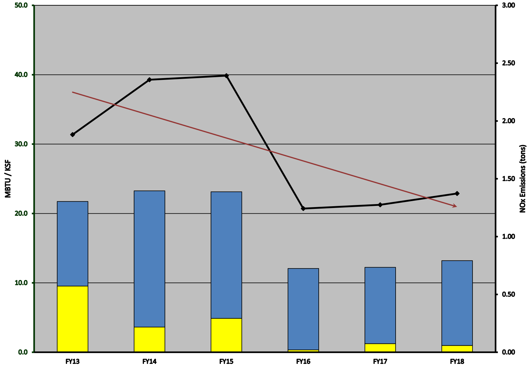
Fuel Use (MBTU/KSF) v. NOx Emissions (FY13 - FY18)
