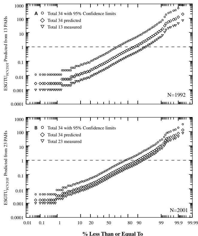
Figure 6-2. Probability distribution of the (A) \Sigma\text{ESBTU}_{\text{FCV},13} and (B) \Sigma\text{ESBTU}_{\text{FCV},23} values for each sediment from the entire database.
