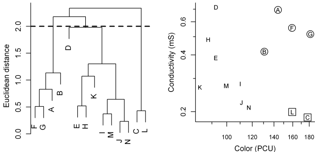
Figure 4-24. Example of agglomerative clustering. Left plot: example of dendrogram using a small subset of the example lake data set. A horizontal line segment on the dendrogram indicates the Euclidean distance between the two branches below that segment. Right plot: Values of log color and log conductivity that correspond with sites shown in the dendrogram. Circles and squares around different letters indicate different classes.
