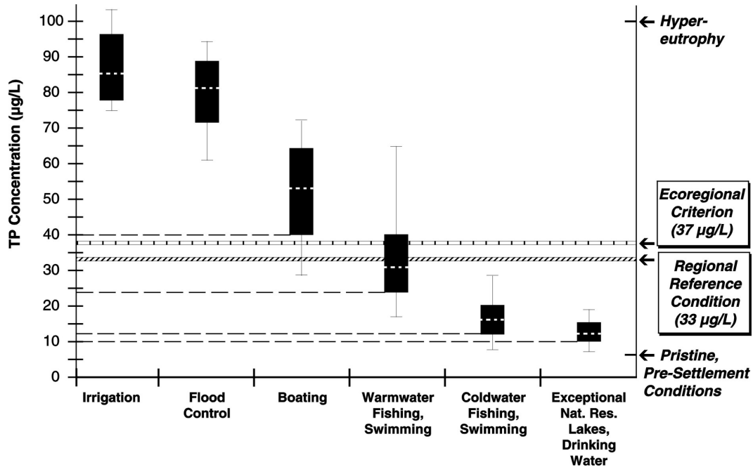
Figure 7.2. Development of TP criteria for select designated uses relative to the reference condition and ecoregional criterion for lakes of a specific size class.
