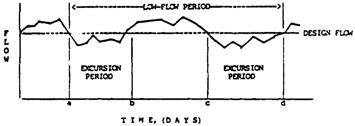
Figure 3-1: Illustration of biologically-based design flow
