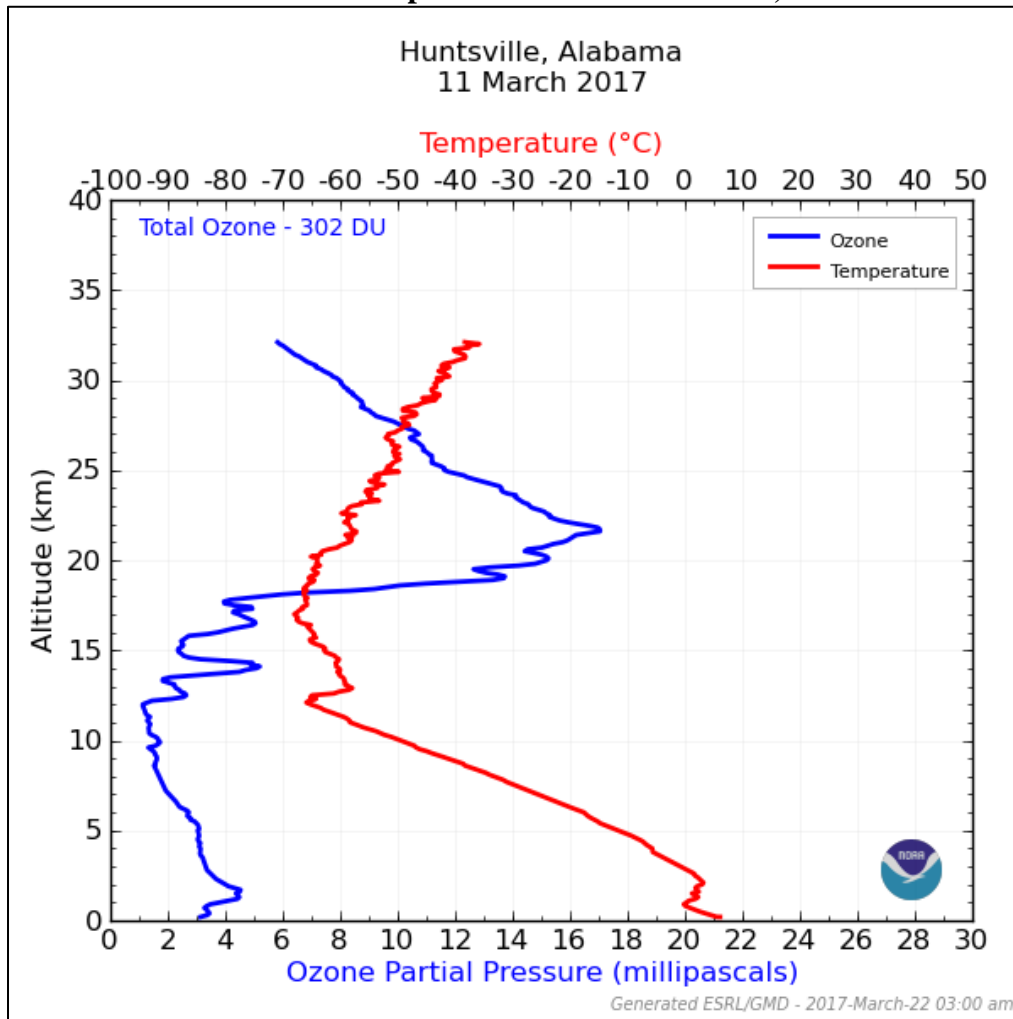
Figure 6c. Ozonesonde data from sample launch from Huntsville, AL 21
