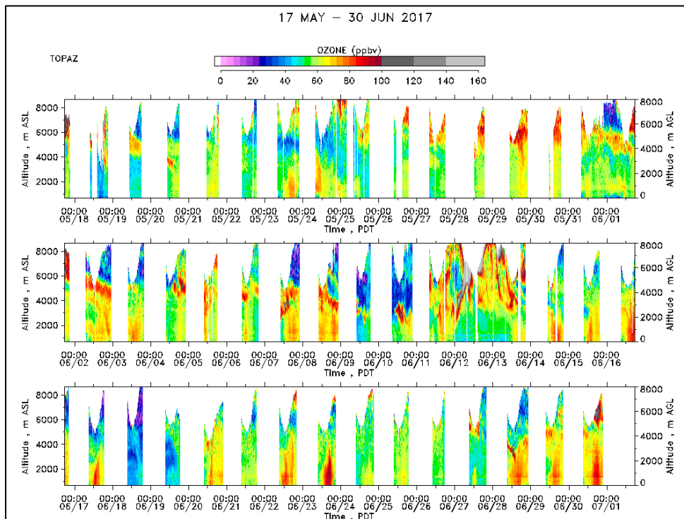
Figure 6d. Time-height ozone cross-sections from May and June 2017 LIDAR measurements near Las Vegas, NV 22
