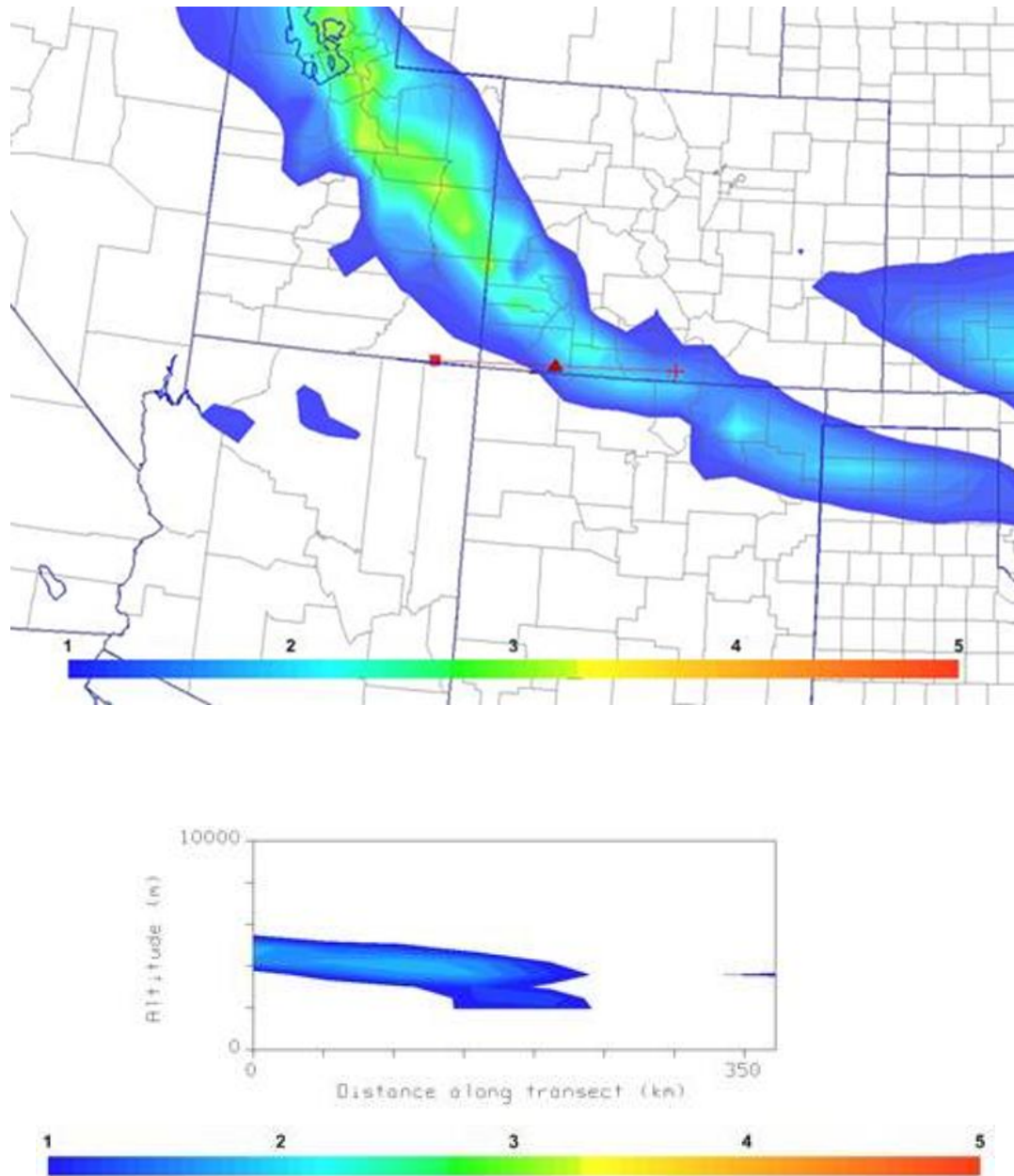
Figure 5c. Plan view (top) and vertical cross-section (bottom) of isentropic potential vorticity ( 10^{-6} \text{ m}^{-2} \text{ s}^{-1} \text{ K kg}^{-1} ) based on reanalysis data for 1200 UTC on April 22, 2017. 18 Horizontal line (red) shows the location of the W-E cross-section. Values of 1 or less are representative of tropospheric air. Higher values are suggestive of stratospheric influence.
