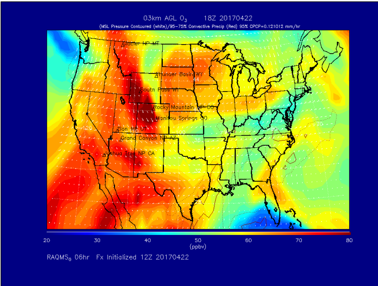
Figure 7b. RAQMS-estimated ozone near the surface at 1800Z on April 22, 2017 28
