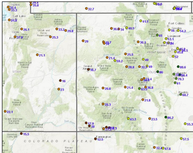
Figure 4aa. Map of relative humidity values in western Colorado region at noon local time for sample case day 14
