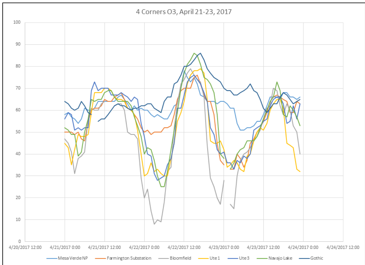
Figure 7a. Time series of ozone at sites in the Four Corners region on April 21-23, 2017 27
