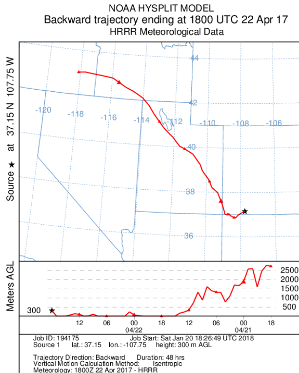
Figure 6f. 48-hour back trajectory from Durango, CO on 1800Z April 22, 2017 25
