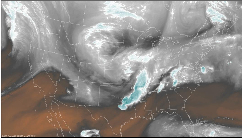
Figure 5a. Water vapor imagery from the GOES-West satellite from sample case day 16
