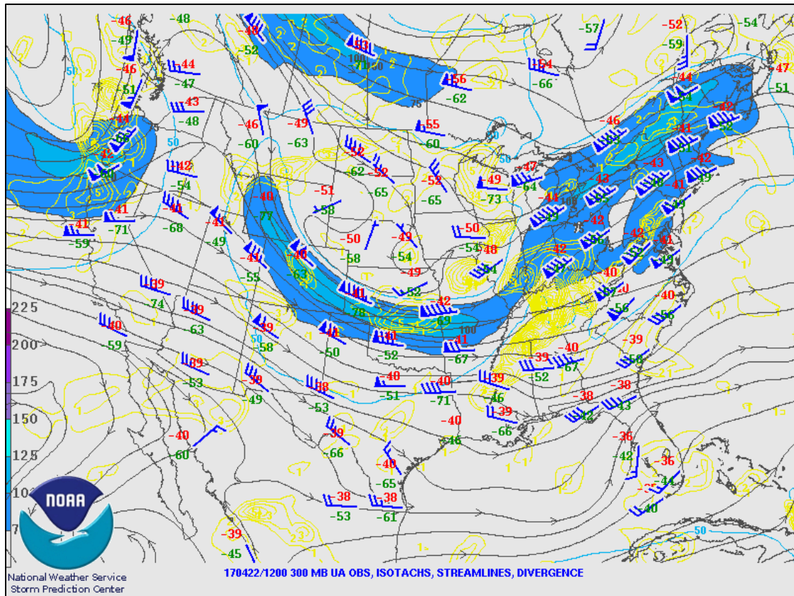
Figure 4b. Map of 300 hPa meteorological observations and isotachs for sample case day 15
