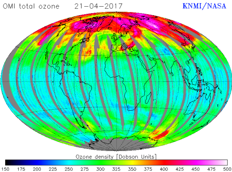
Figure 5b. Map of satellite-estimated total column ozone data from the day before the case event 17
