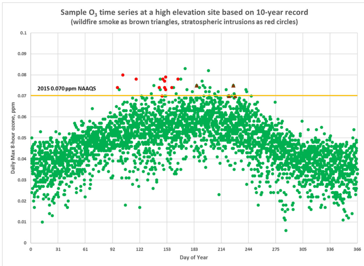
Figure 2. Sample historical comparison analyses showing how previous non-event days compare against event-influenced days. Data is from U.S. Air Force Academy site from 2008 to 2017
