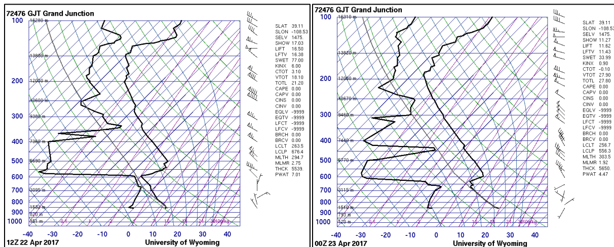
Figures 6a and 6b. Skew-T diagrams for 1200Z (left) April 22, 2017 and 0000Z (right) April 23, 2017, at Grand Junction, CO 20
