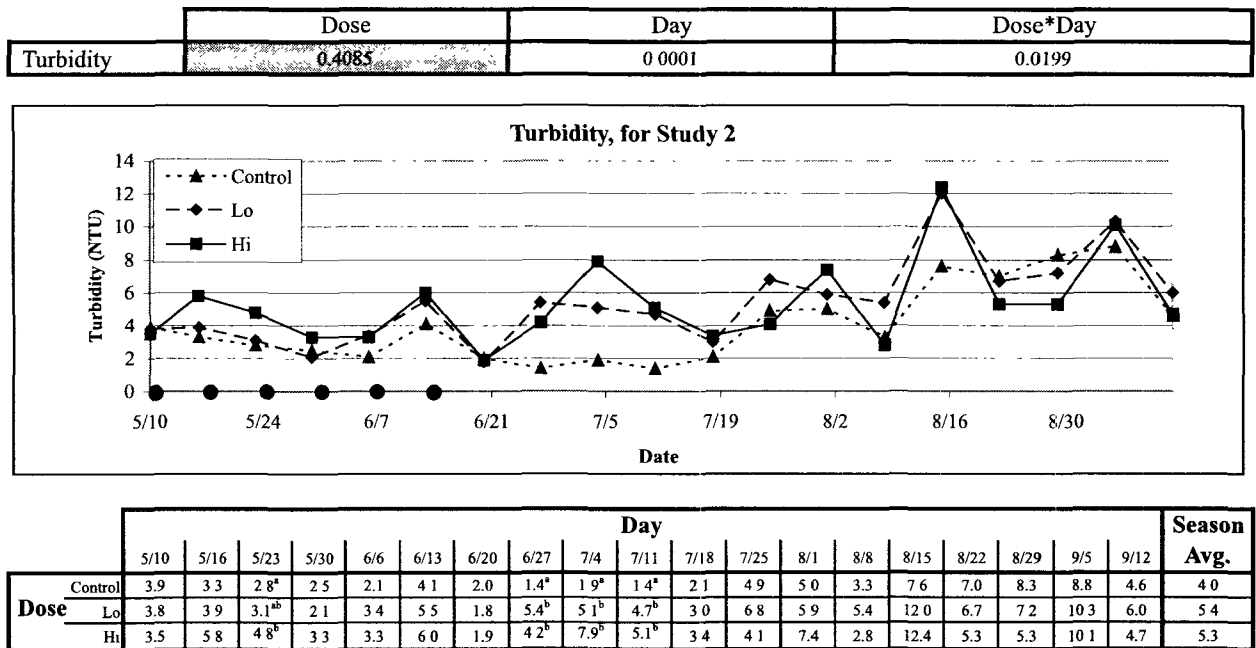
Figure 48. Changes in turbidity over time. This combination of tables and a graph presents the data and statistical information pertaining to turbidity (NTU). The upper table presents probabilities that dose, day, and interactions of dose and day influenced turbidity in ANOVA of rank-transformed data. Darkened values are not significant ( p > 0.05 ). The graph is a plot of turbidity over the experimental season pooled by treatment. Dark circles indicate dose dates. The lower table lists LS Means (NTU) represented in the graph, along with statistical information based on the rank transformed data. Within a column, values sharing a letter are not significantly different ( p > 0.05 ). In columns without letters, values are not significantly different.
