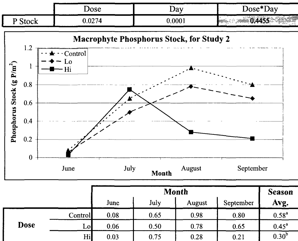
Figure 36. Changes in macrophyte phosphorus stock over time. The upper table presents probabilities that dose, day, and interactions of dose and day influenced P stock in ANOVA of rank-transformed data. Darkened values are not significant ( p>0.05 ). The graph is a plot of P stock over the experimental season pooled by treatment. The final dose occurred one week subsequent to June samples. The lower table lists LS Means ( \text{g P/m}^2 ) represented in the graph, along with statistical information based on the rank transformed data. Within a column, values sharing a letter are not significantly different ( p>0.05 ). In columns without letters, values are not significantly different.
