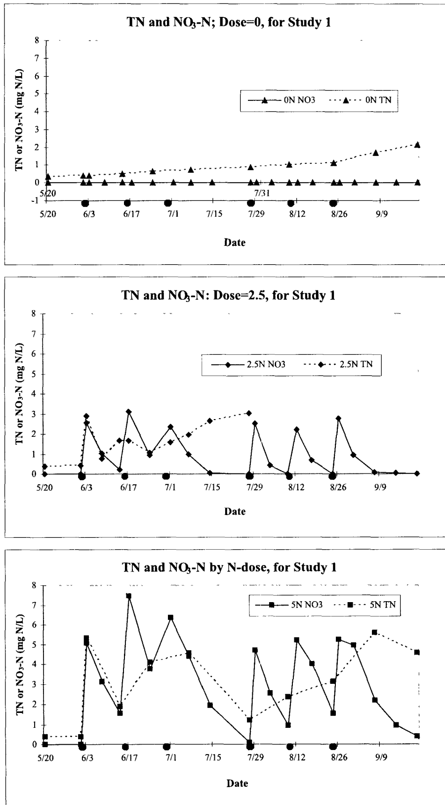
Figure 11. Total and nitrate nitrogen over the season pooled by N-dose level. Nitrate values for 0N are not visible due to scale. Dark circles on X axis mark dose dates.
