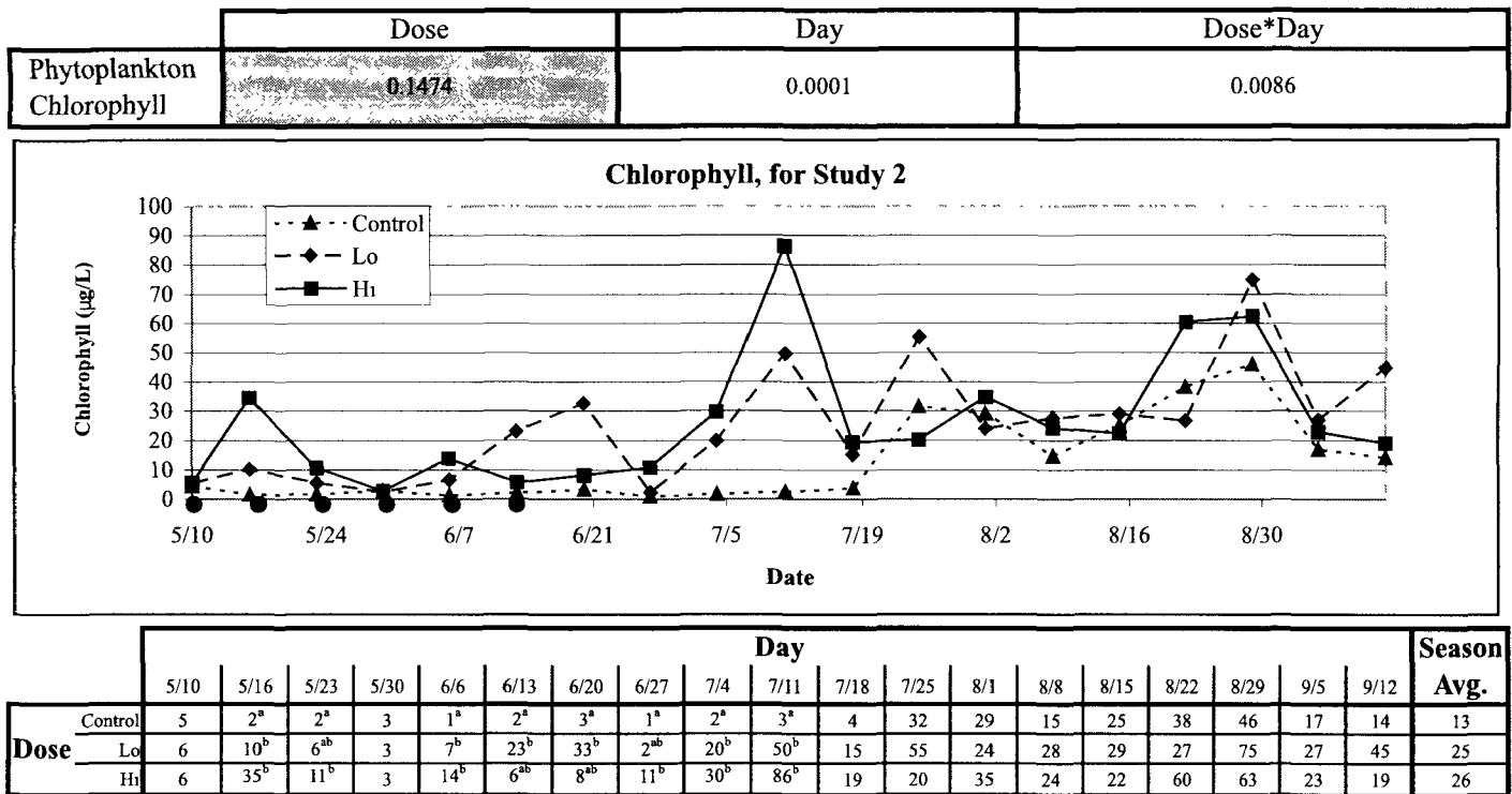
Figure 49. Changes in phytoplankton chlorophyll concentrations over time. The upper table presents probabilities that dose, day, and interactions of dose and day influenced Chl in ANOVA of rank-transformed data. Darkened values are not significant ( p > 0.05 ). The graph is a plot of Chl over the experimental season pooled by treatment. Dark circles on X axis indicate dose dates. The lower table lists LS Means ( \text{mg/L} ) represented in the graph, along with statistical information based on the rank transformed data. Within a column, values sharing a letter are not significantly different ( p > 0.05 ). In columns without letters, values are not significantly different.
