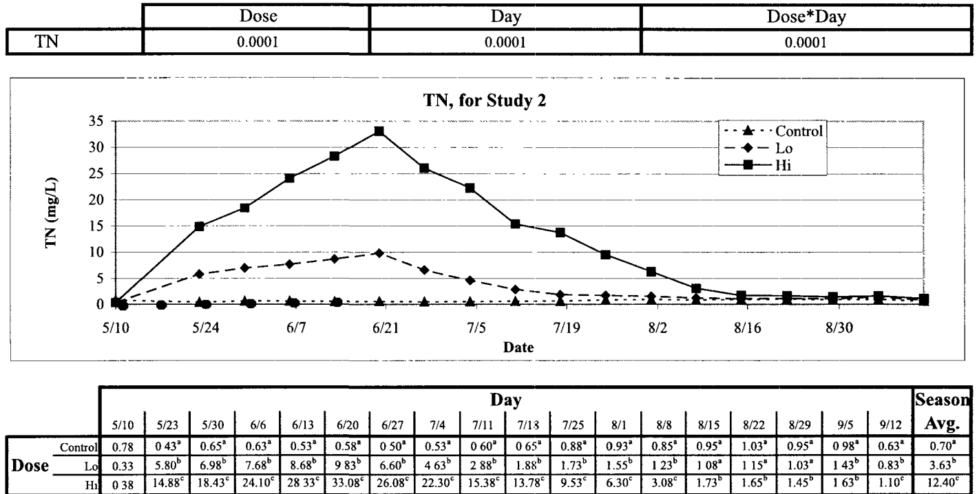
Figure 39. Changes in total nitrogen concentrations over time. The upper table presents probabilities that dose, day, and interactions of dose and day influenced TN in ANOVA of rank-transformed data. The graph is a plot of TN over the experimental season pooled by treatment. Dark circles indicate dose dates. The lower table lists LS Means (mg/L) represented in the graph, along with statistical information based on the rank transformed data. Within a column, values sharing a letter are not significantly different ( p > 0.05 ). In columns without letters, values are not significantly different.
