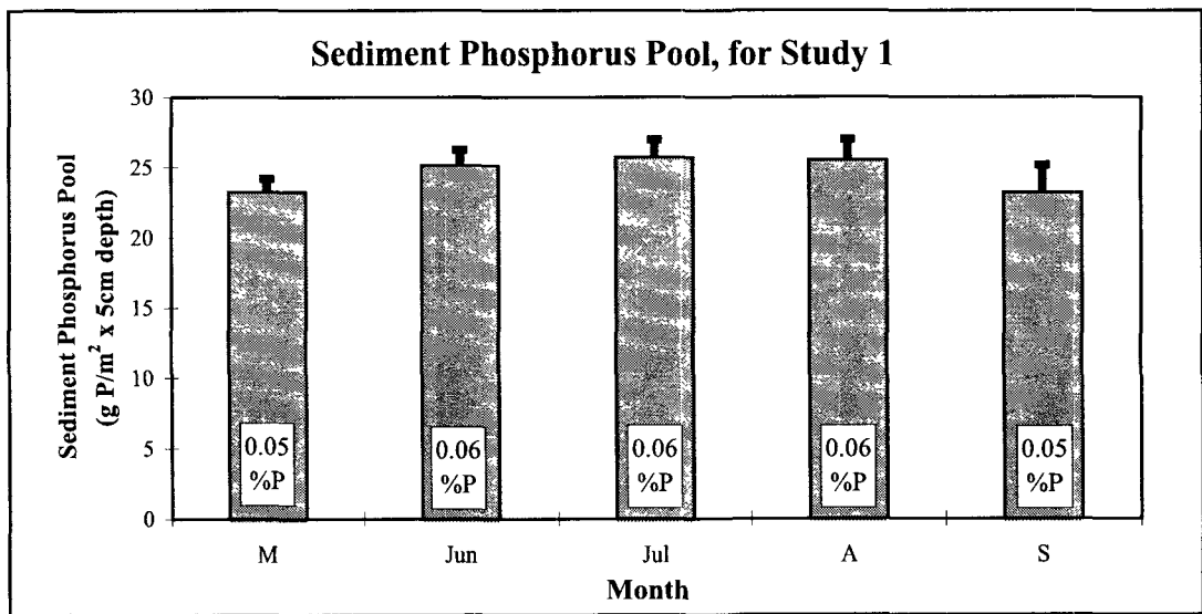
Figure 28. Changes in sediment phosphorus pool over time. The table presents probabilities that dose, day, and interactions of dose and day influenced P content in sediments in ANOVA of rank-transformed data. Darkened values are not significant ( p > 0.05 ). The graph is a plot of the estimated pool of P in the sediments for an area of 1 m 2 and a depth of 5 cm. Because treatment influences were not significant, monthly values are presented as averages of all treatments. The average %P in sediments is shown within the column for each month.
