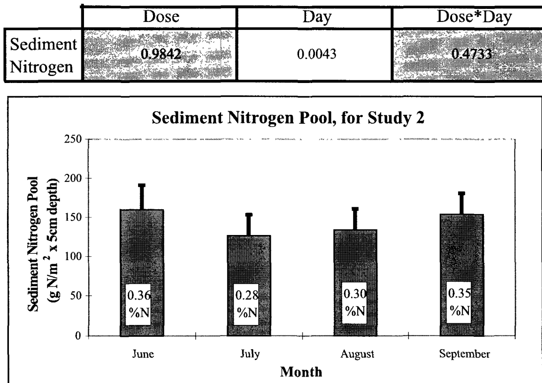
Figure 55. Changes in the sediment nitrogen pool over time. The table presents probabilities that dose, day, and interactions of dose and day influenced N content in sediments in ANOVA of rank-transformed data. Darkened values are not significant ( p > 0.05 ). The graph is a plot of the estimated pool of N in the sediments for an area of 1 m^2 and a depth of 5 cm. Because treatment influences were not significant, monthly values are presented as averages of all treatments. The average %N in sediments is shown within the column for each month.
