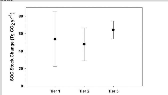
Figure A-12: Comparison of Estimated Soil Organic C Stock Changes and Uncertainties using Tier 1 (IPCC 2006), Tier 2 (Ogle et al. 2003, 2006) and Tier 3 Methods
