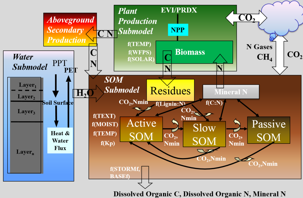
Figure A-7: DayCent Model Flow Diagram
