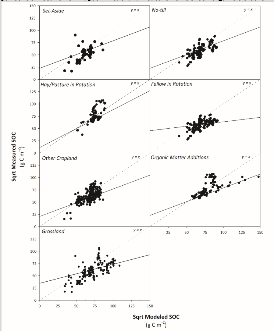
Figure A-11: Comparisons of Results from DayCent Model and Measurements of Soil Organic C Stocks
