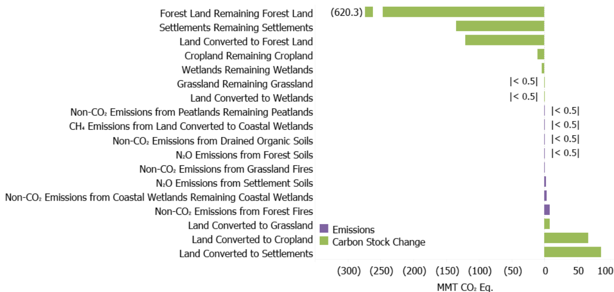
1 Figure 6-1: 2017 LULUCF Chapter Greenhouse Gas Sources and Sinks (MMT CO 2 Eq.)
