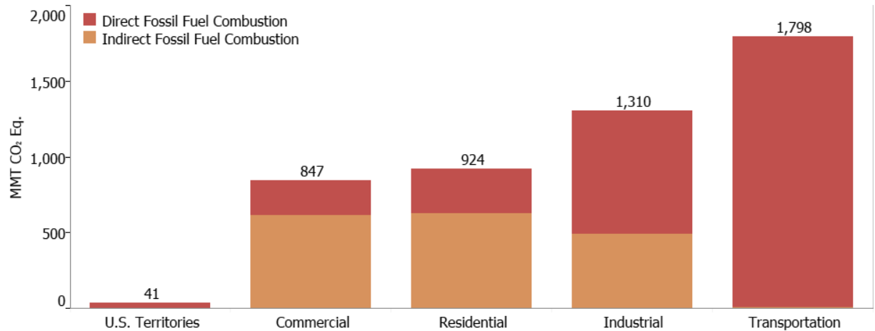
Figure ES-7: 2017 End-Use Sector Emissions of CO 2 from Fossil Fuel Combustion (MMT CO 2 Eq.)
