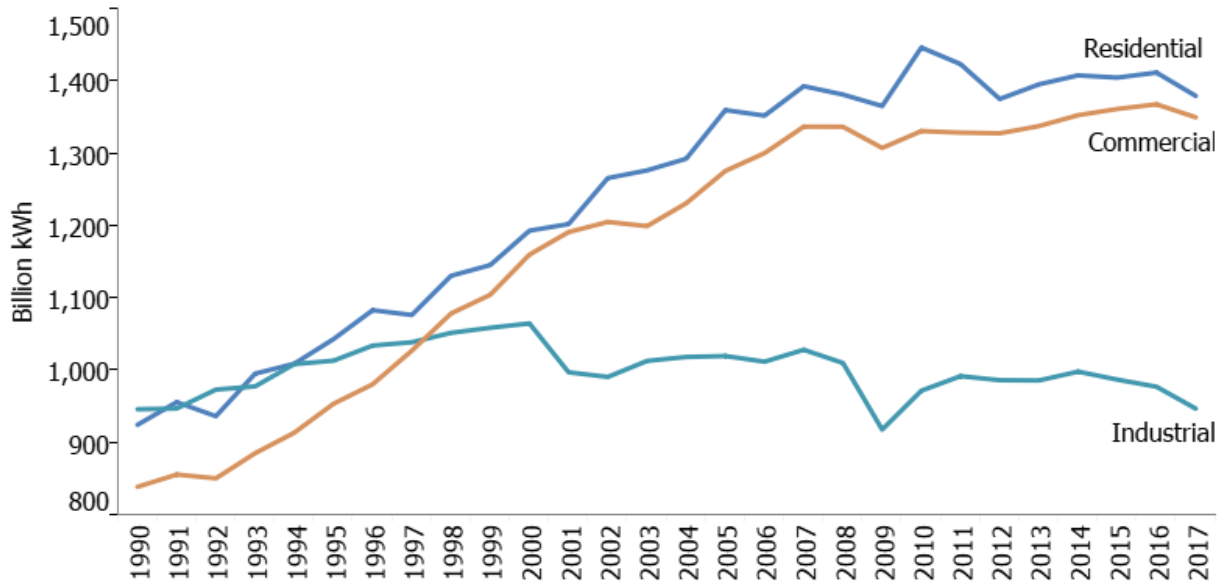
Figure 3-9: Electric Power Retail Sales by End-Use Sector (Billion kWh)
