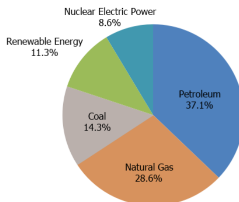
Figure ES-13: 2017 U.S. Energy Consumption by Energy Source (Percent)
