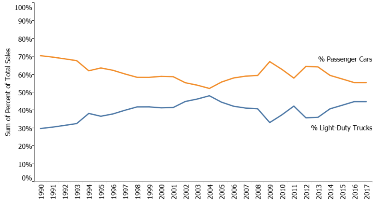
Figure 3-14: Sales of New Passenger Cars and Light-Duty Trucks, 1990–2017 (Percent)
