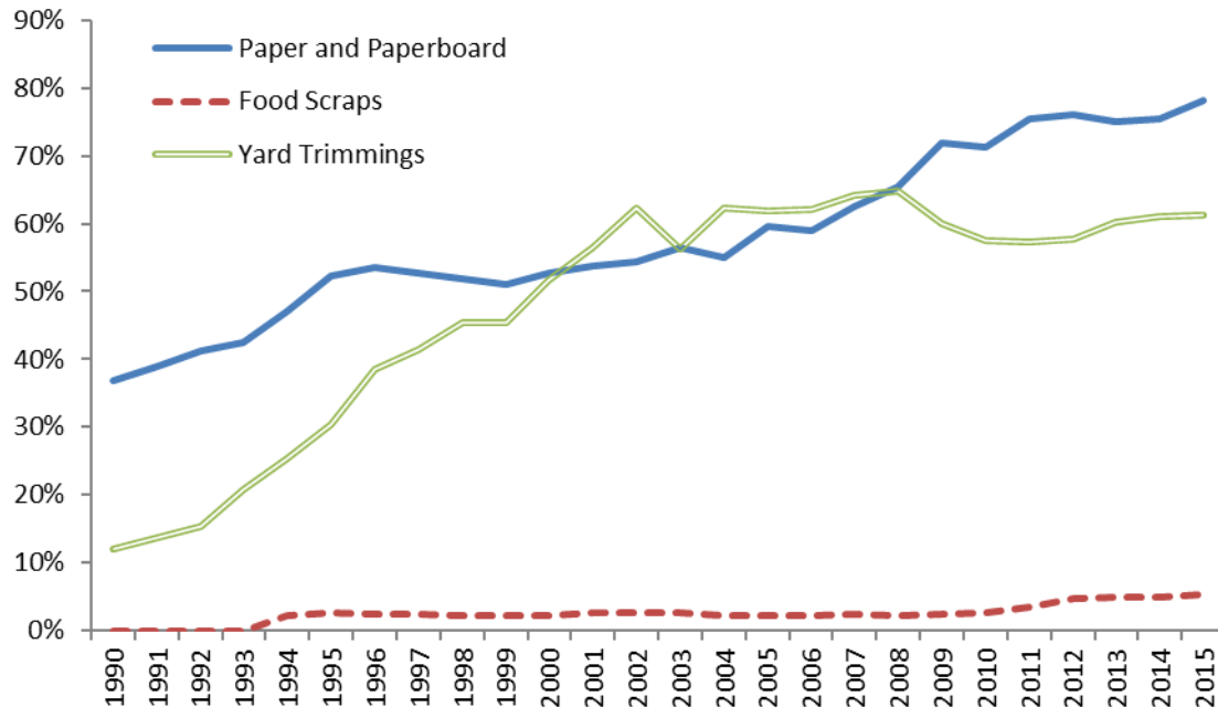
Figure 7-4: Percent of Degradable Materials Diverted from Landfills from 1990 to 2015 (Percent)
