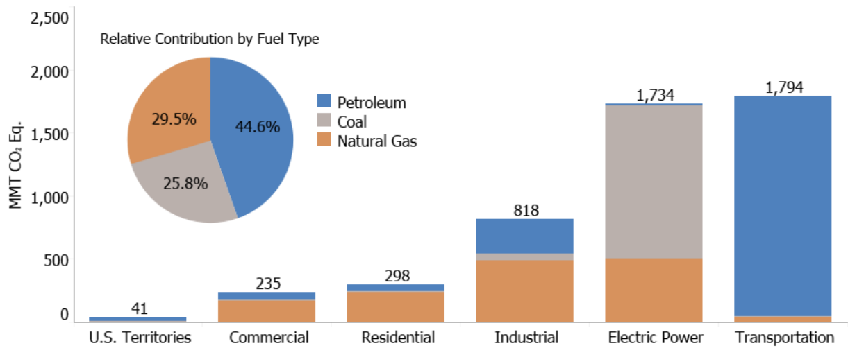
Figure 3-5: 2017 CO 2 Emissions from Fossil Fuel Combustion by Sector and Fuel Type (MMT CO 2 Eq.)
