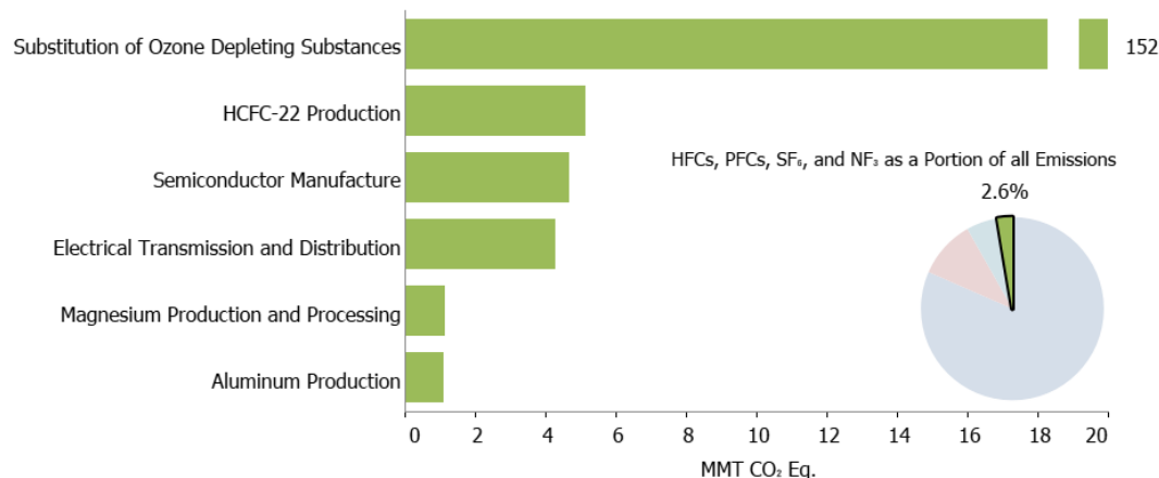
Figure ES-11: 2017 Sources of HFCs, PFCs, SF 6 , and NF 3 Emissions (MMT CO 2 Eq.)
