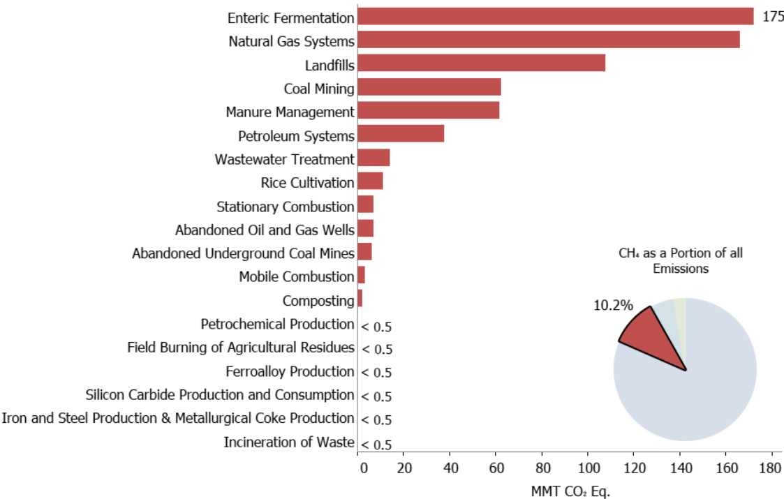
Figure ES-9: 2017 Sources of CH 4 Emissions (MMT CO 2 Eq.)
