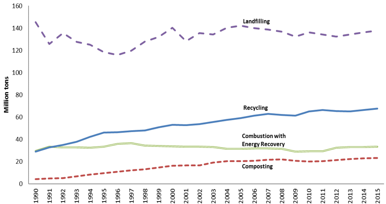
Figure 7-3: MSW Management Trends from 1990 to 2015
