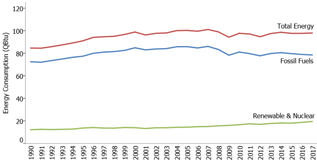
Figure 3-4: U.S. Energy Consumption (Quadrillion Btu)
