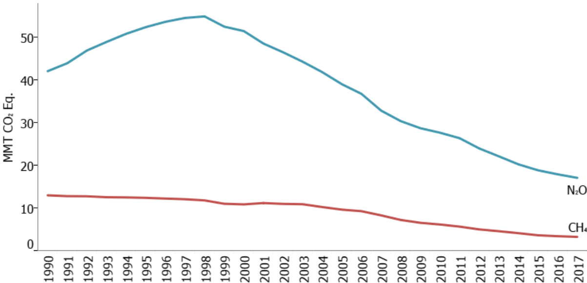
Figure 3-15: Mobile Source CH 4 and N 2 O Emissions (MMT CO 2 Eq.)
