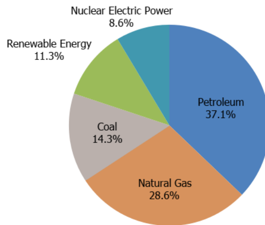
Figure 3-3: 2017 U.S. Energy Consumption by Energy Source (Percent)
