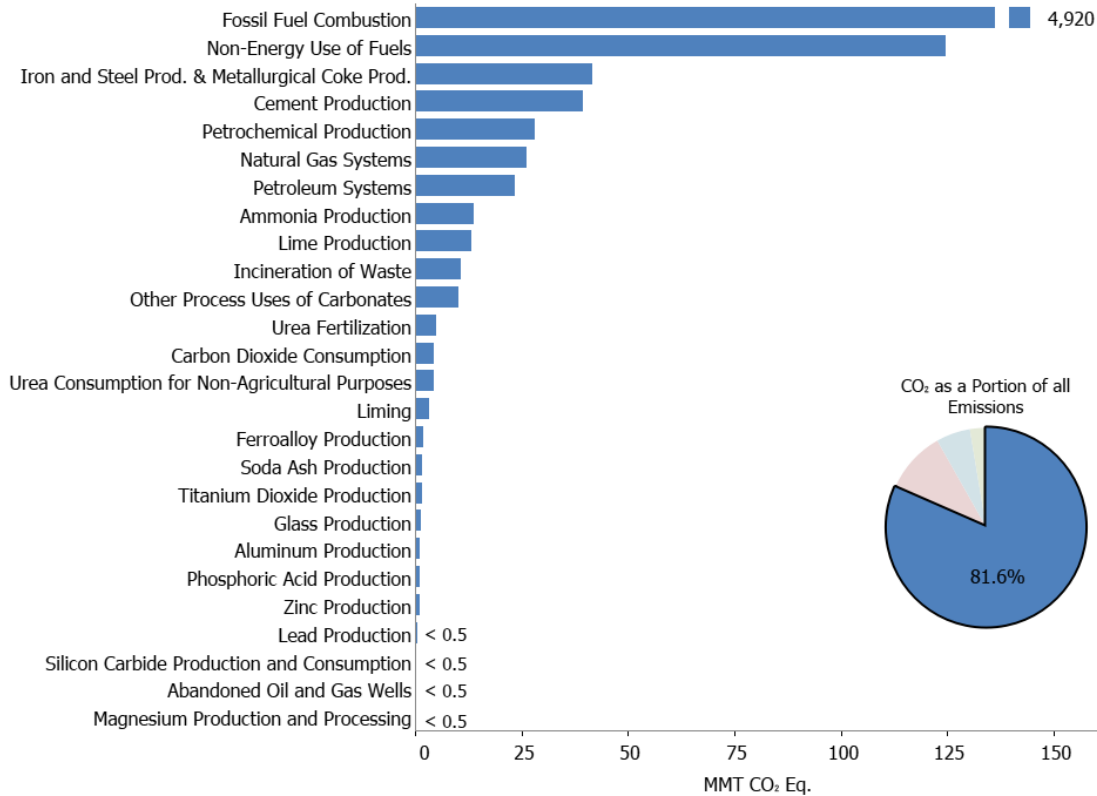
Figure ES-5: 2017 Sources of CO 2 Emissions (MMT CO 2 Eq.)
