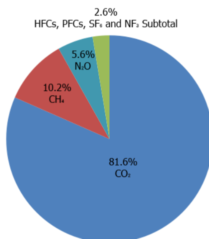
Figure ES-4: 2017 U.S. Greenhouse Gas Emissions by Gas (Percentages based on MMT CO 2 Eq.)
