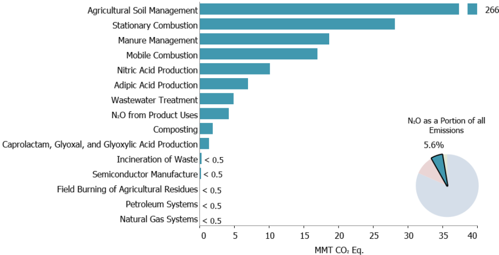
Figure ES-10: 2017 Sources of N 2 O Emissions (MMT CO 2 Eq.)
