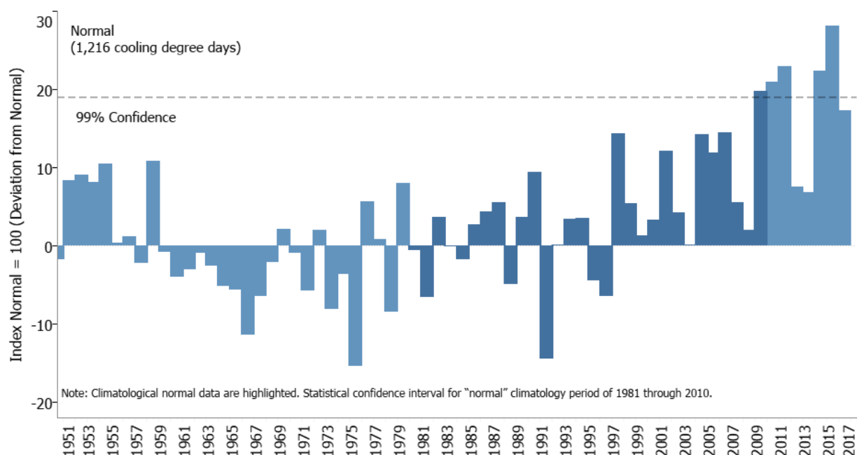
Figure 3-7: Annual Deviations from Normal Cooling Degree Days for the United States (1950–2017, Index Normal = 100)
