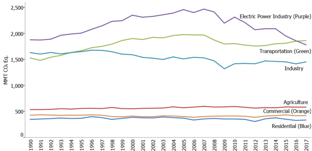
Figure ES-14: U.S. Greenhouse Gas Emissions Allocated to Economic Sectors (MMT CO 2 Eq.)
