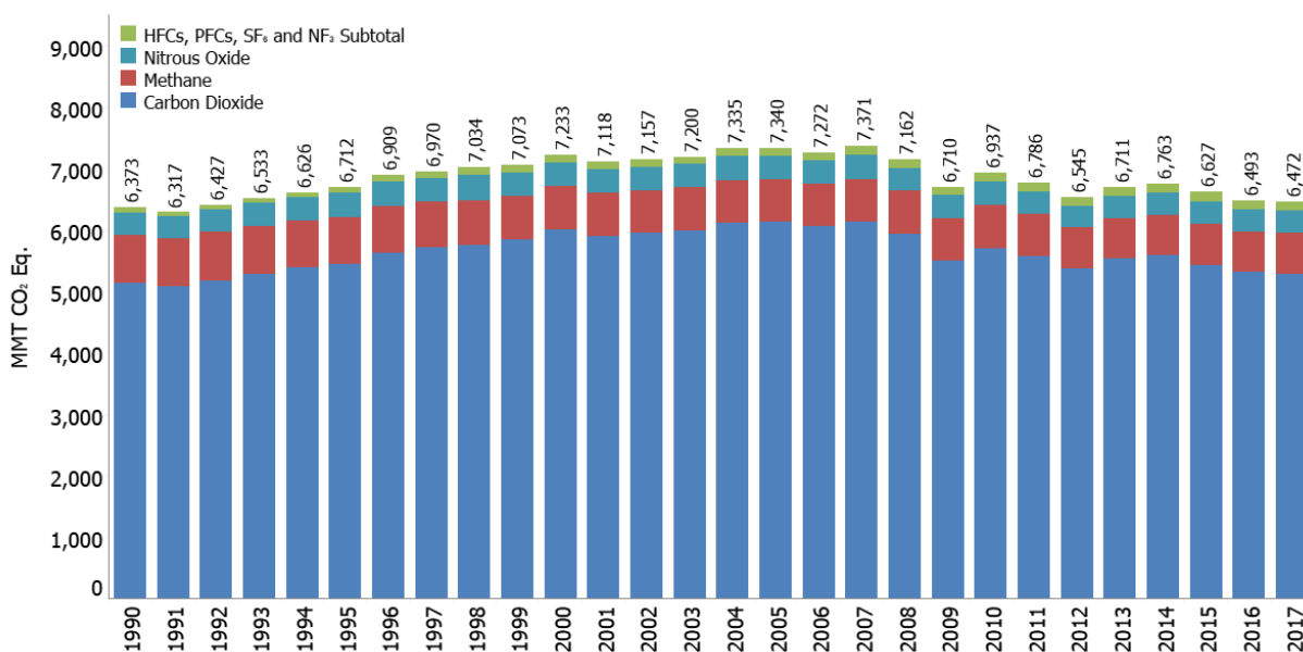
Figure ES-1: Gross U.S. Greenhouse Gas Emissions by Gas (MMT CO 2 Eq.)
