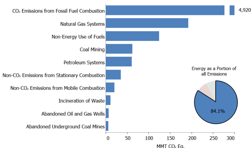
Figure 3-1: 2017 Energy Chapter Greenhouse Gas Sources (MMT CO 2 Eq.)
