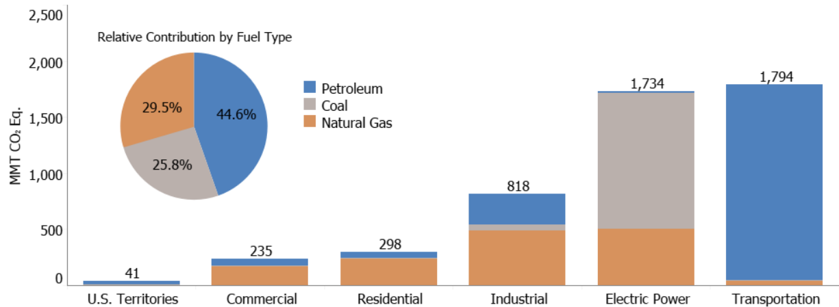
Figure ES-6: 2017 CO 2 Emissions from Fossil Fuel Combustion by Sector and Fuel Type (MMT CO 2 Eq.)
