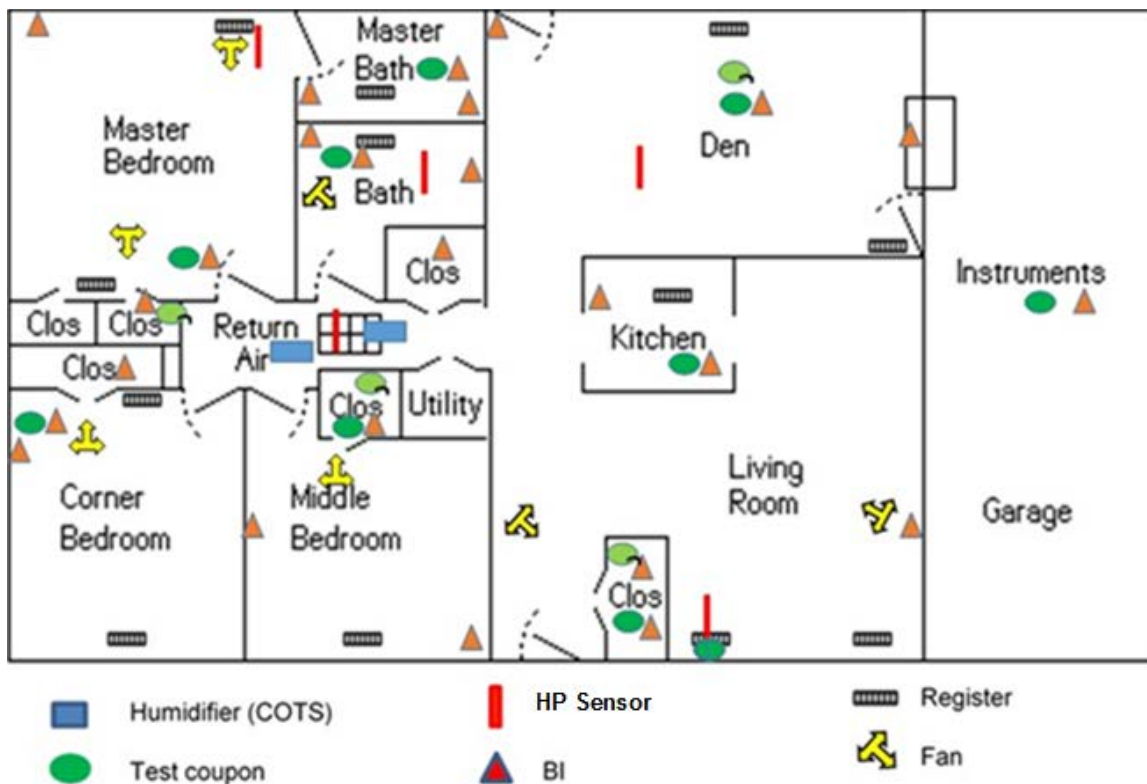
Figure 5-36. CTH Equipment and Sampling Locations for Test 5
