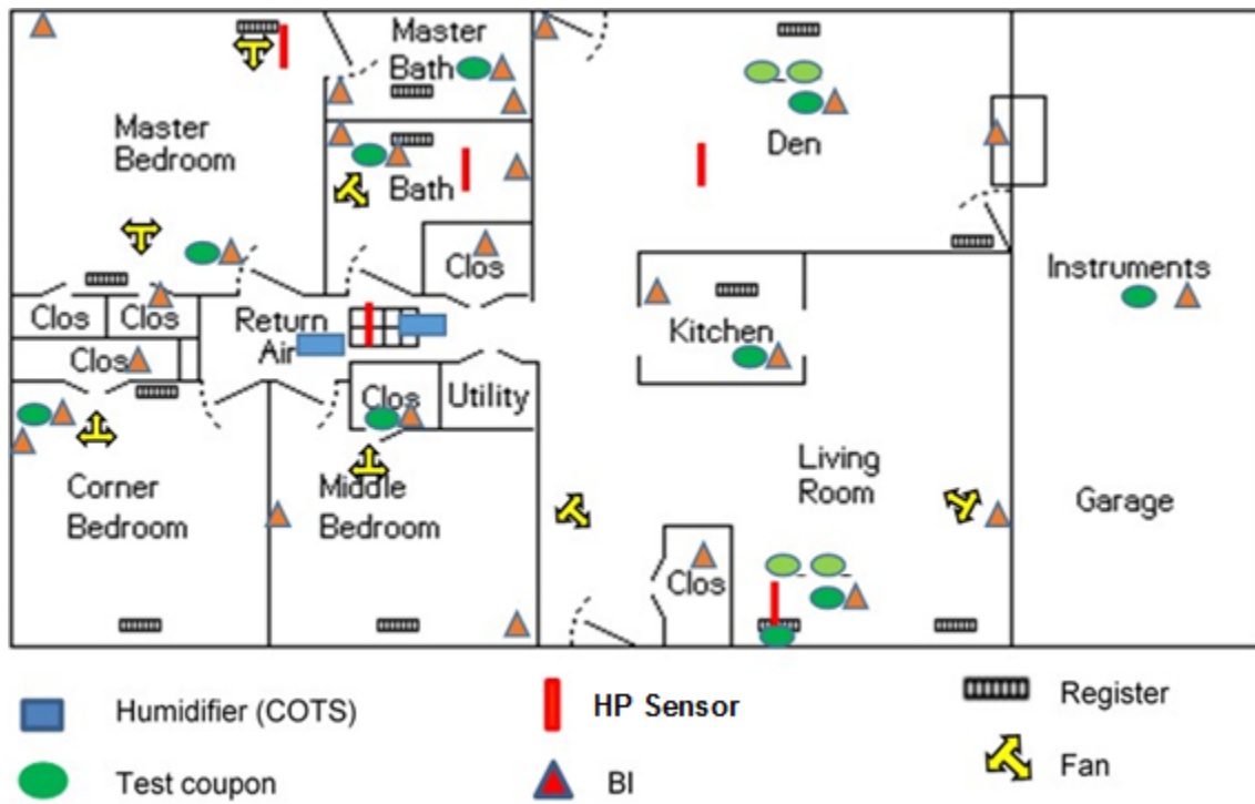
Figure 5-29. CTH Equipment and Sampling Locations for Test 4
