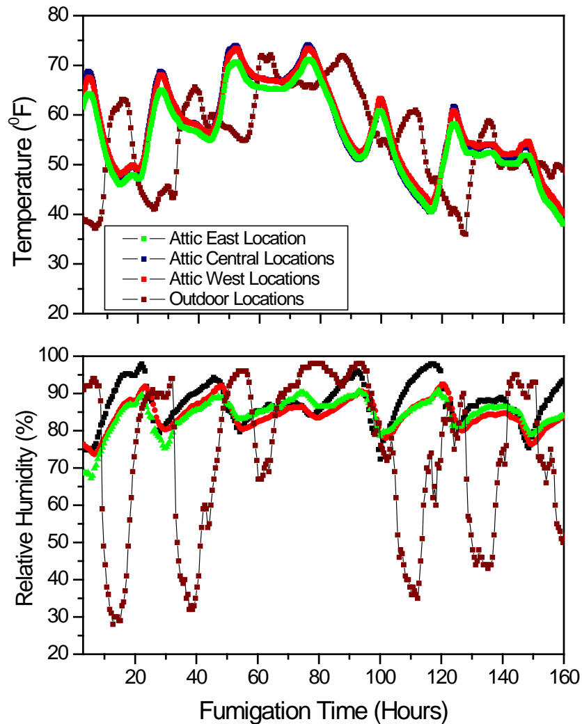
Figure 5-20. Test 2 Temporal RH in Attic
