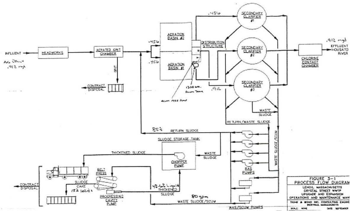
Figure 2 Lenox WWTP Process Flow Schematic
