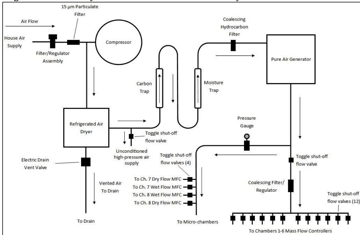
Figure 1. Clean Air System for Small Chamber Laboratory
