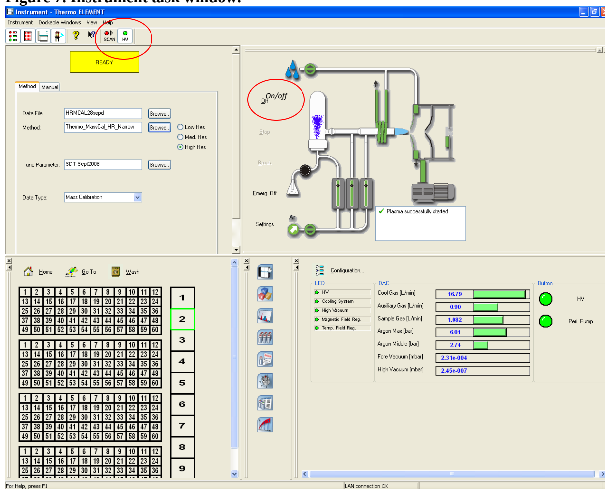
Figure 7. Instrument task window.
