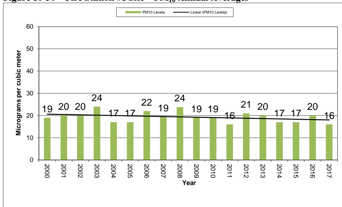
Figure 10-30 – Fire Station #1 Site – PM 10 Annual Averages
