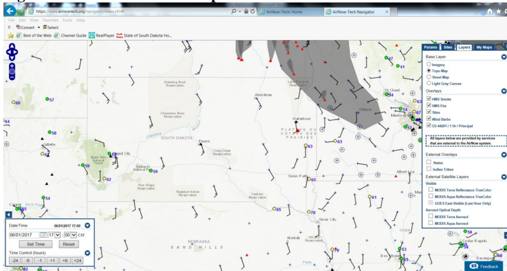
Figure 9-34 - AirNow Tech Map for 6/1/17
