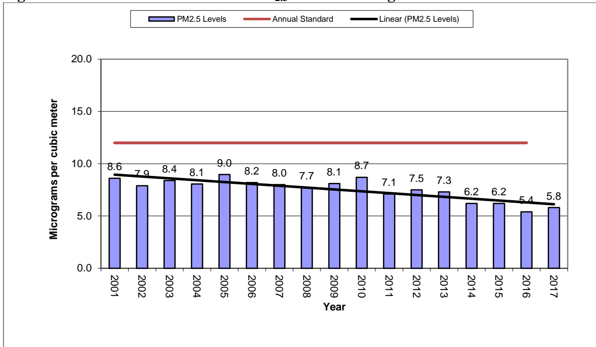
Figure 10-31 – Fire Station #1 Site – PM 2.5 Annual Averages
