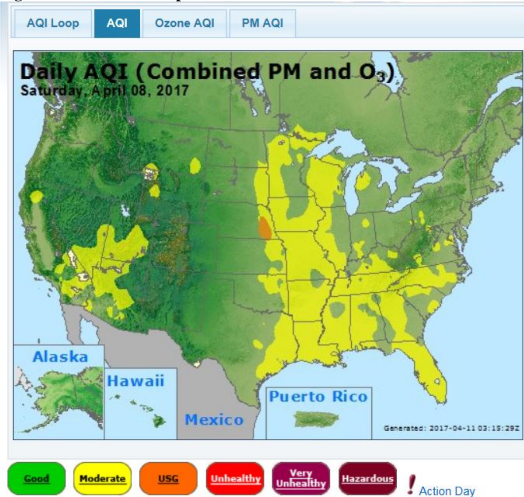
Figure 9-11 – AirNow Map for 4/8/17
