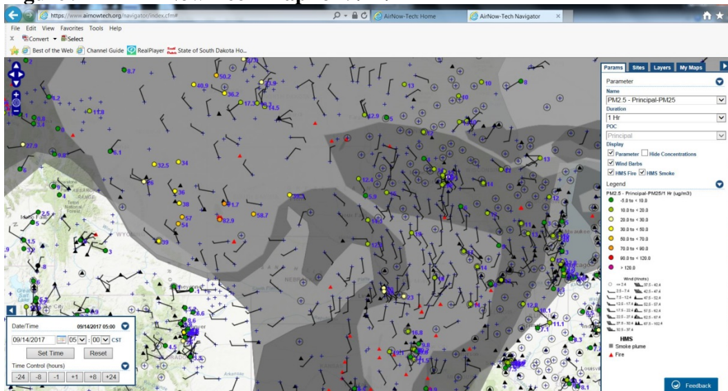
Figure 9-22 - AirNow Tech Map for 9/14/17
