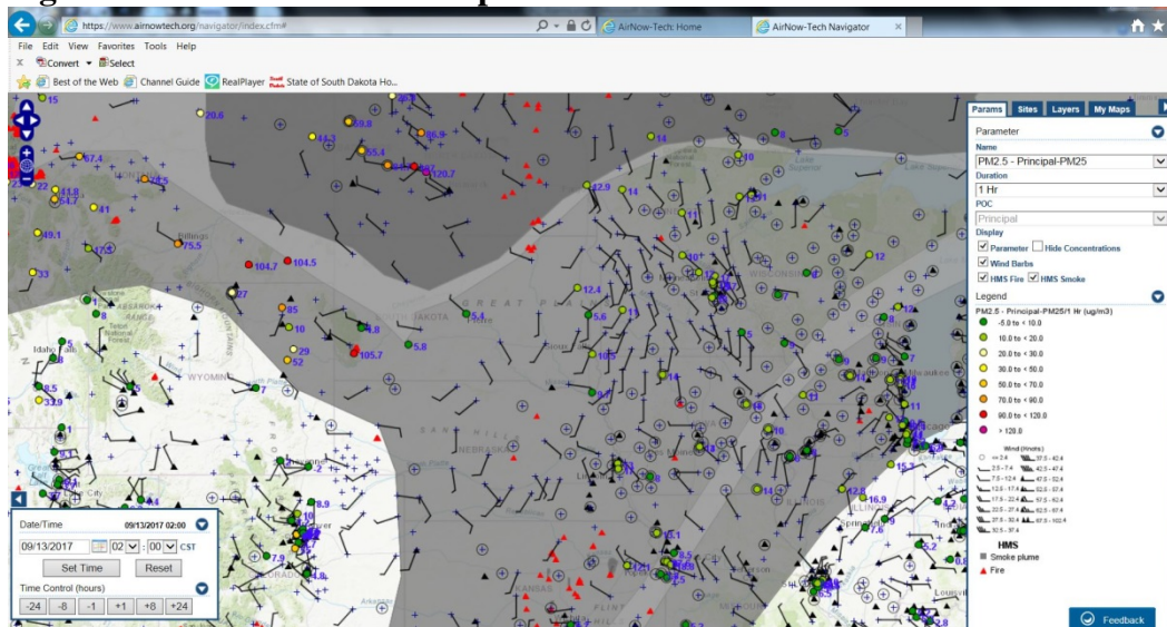
Figure 9-20 - AirNow Tech Map for 9/13/17
