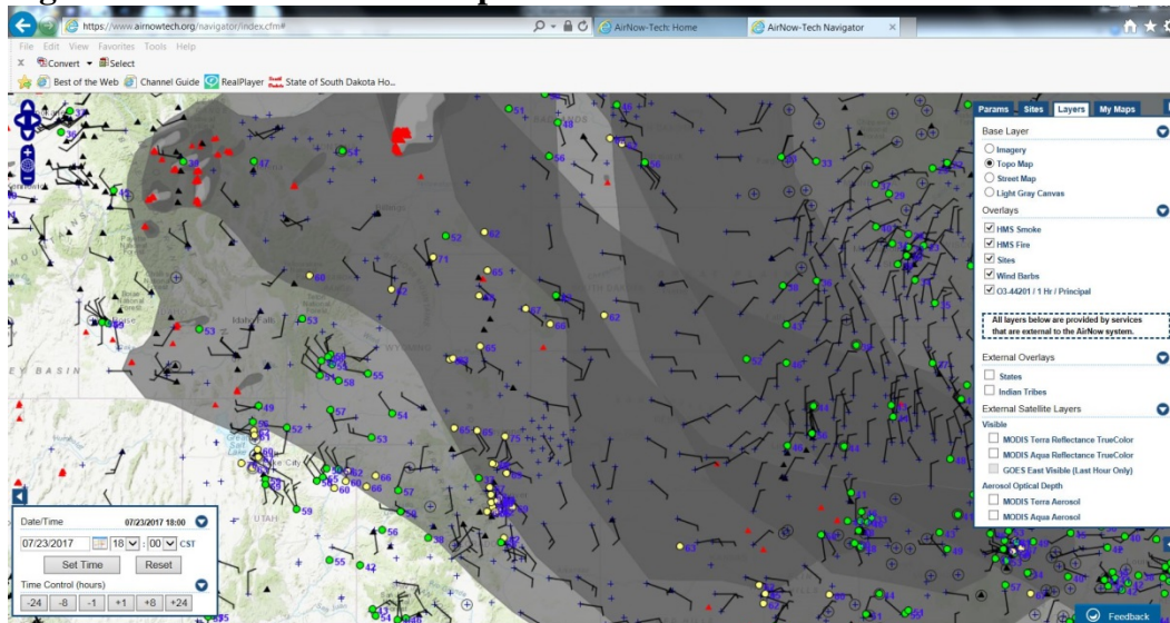
Figure 9-66 - AirNow Tech Map for 7/23/17
