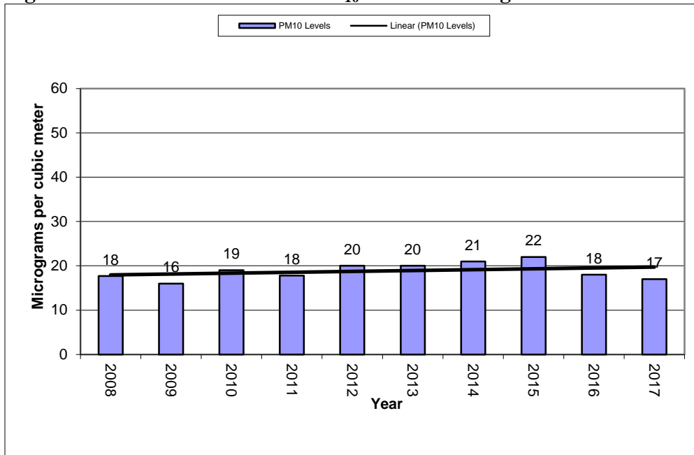
Figure 10-23 – SD School Site – PM 10 Annual Averages
