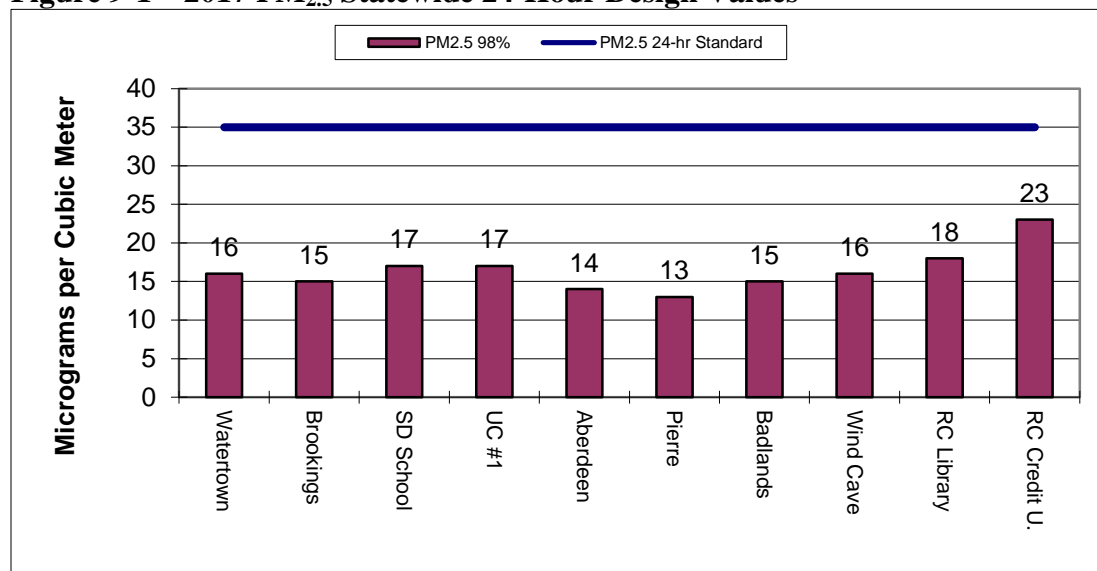
Figure 9-1 – 2017 PM 2.5 Statewide 24-Hour Design Values
