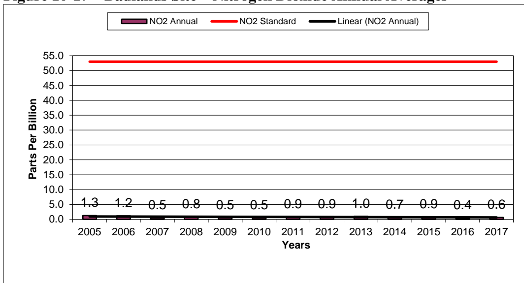
Figure 10-17 – Badlands Site – Nitrogen Dioxide Annual Averages
