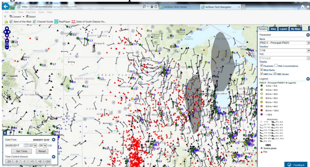
Figure 9-12 – AirNow Tech Map for 4/8/17
