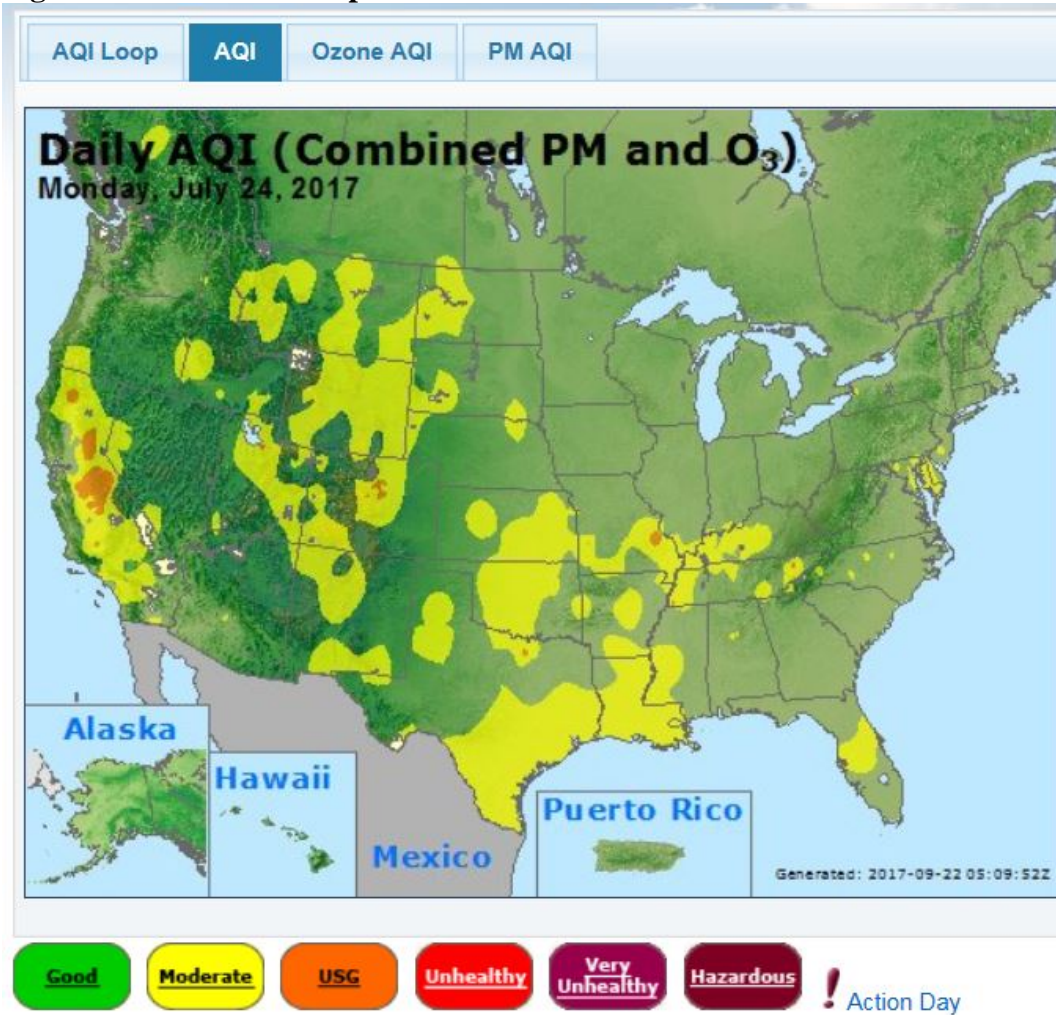
Figure 9-67 - AirNow Map for 7/24/17
