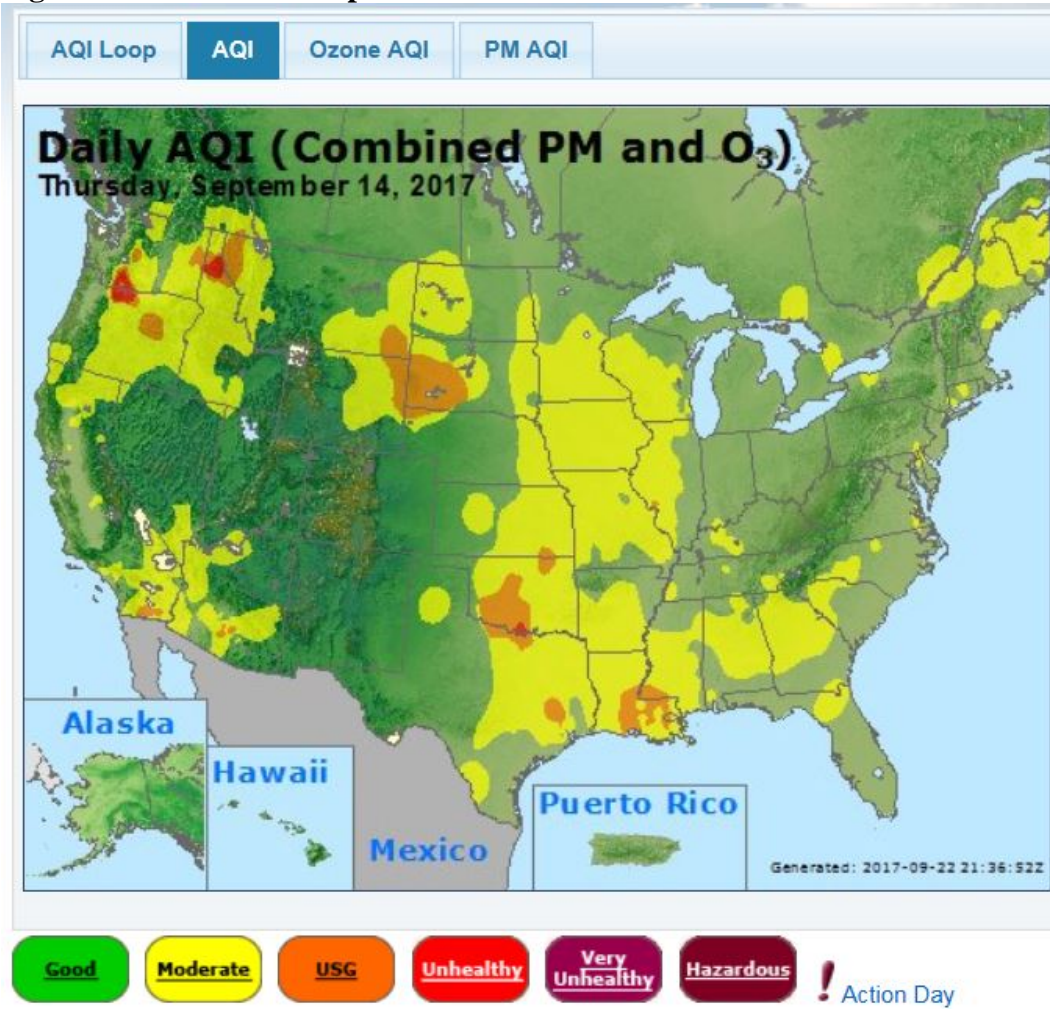
Figure 9-21 - AirNow Map for 9/14/17
