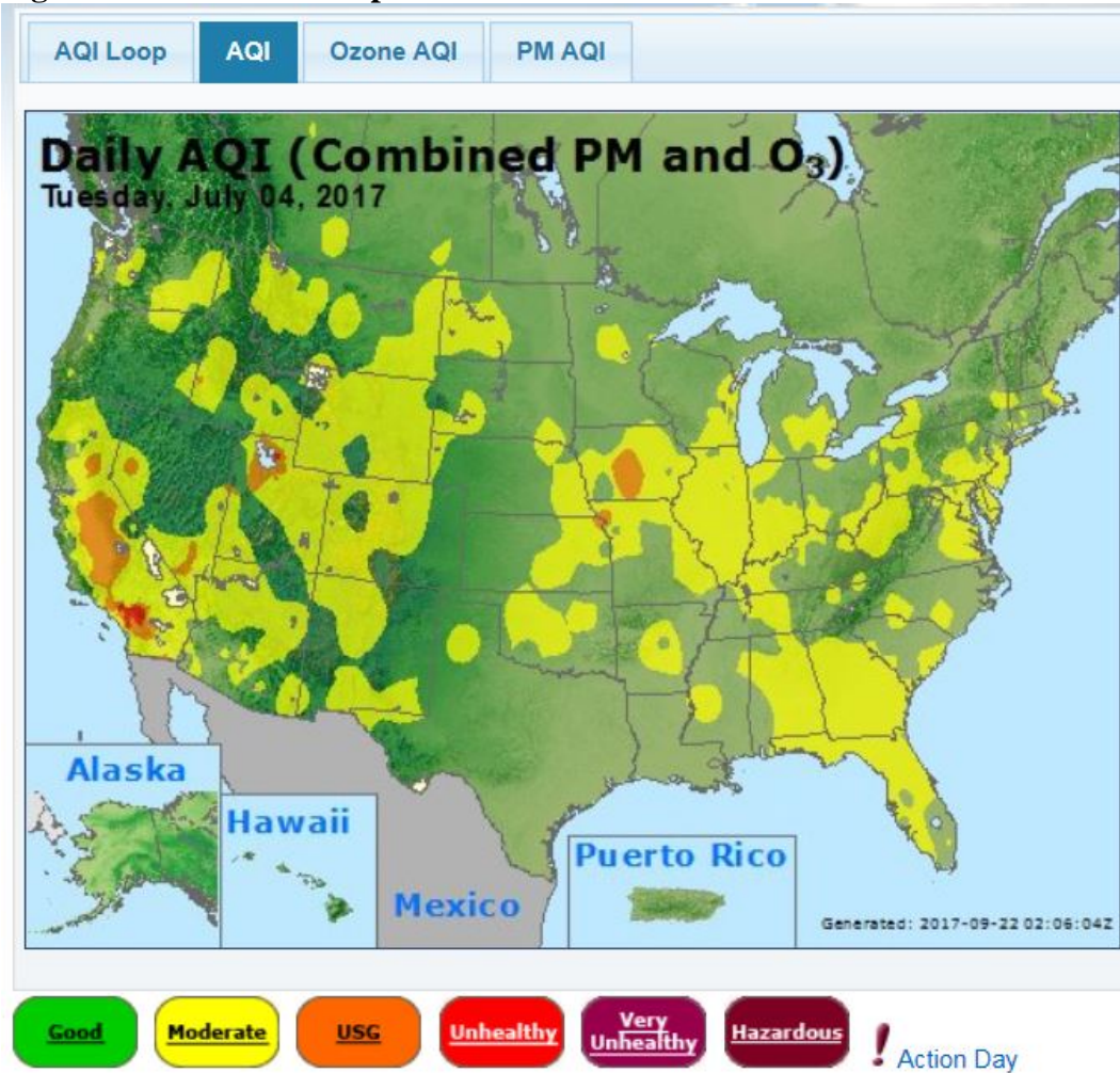
Figure 9-51 - AirNow Map for 7/4/17
