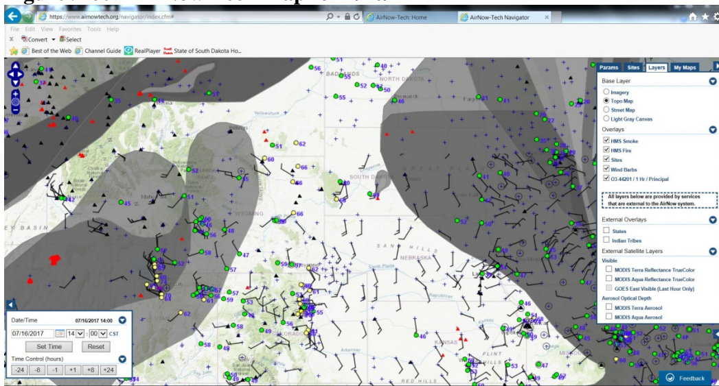
Figure 9-60 - AirNow Tech Map for 7/16/17
