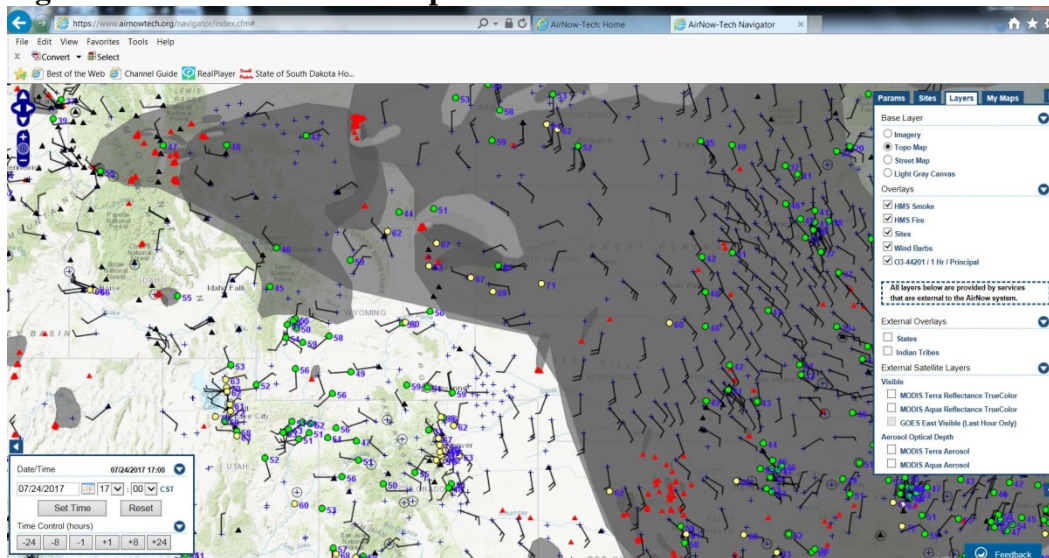
Figure 9-68 - AirNow Tech Map for 7/24/17
