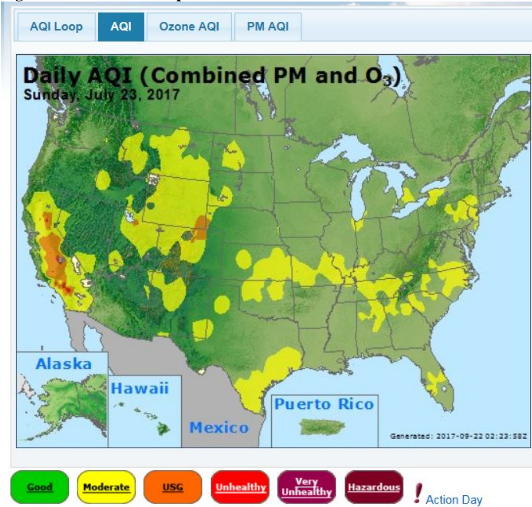
Figure 9-66 - AirNow Tech Map for 7/23/17
