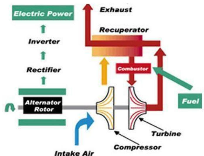
Figure 1: Microturbine Flow Diagram
