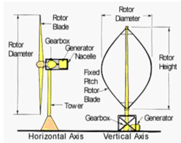
Figure 2: Two Wind Turbine Configurations.
