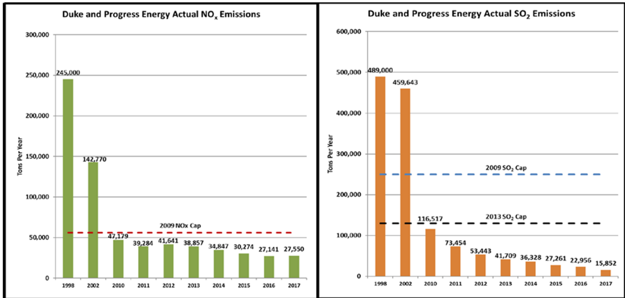
Figure 1. Clean Smokestacks Act Emissions Reductions
