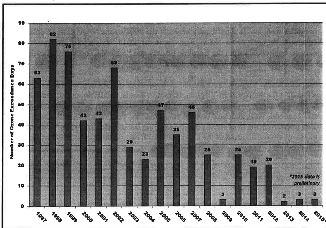
Figure 3: Virginia Ozone Exceedence Day Trends. 2008 Ozone NAAQS
