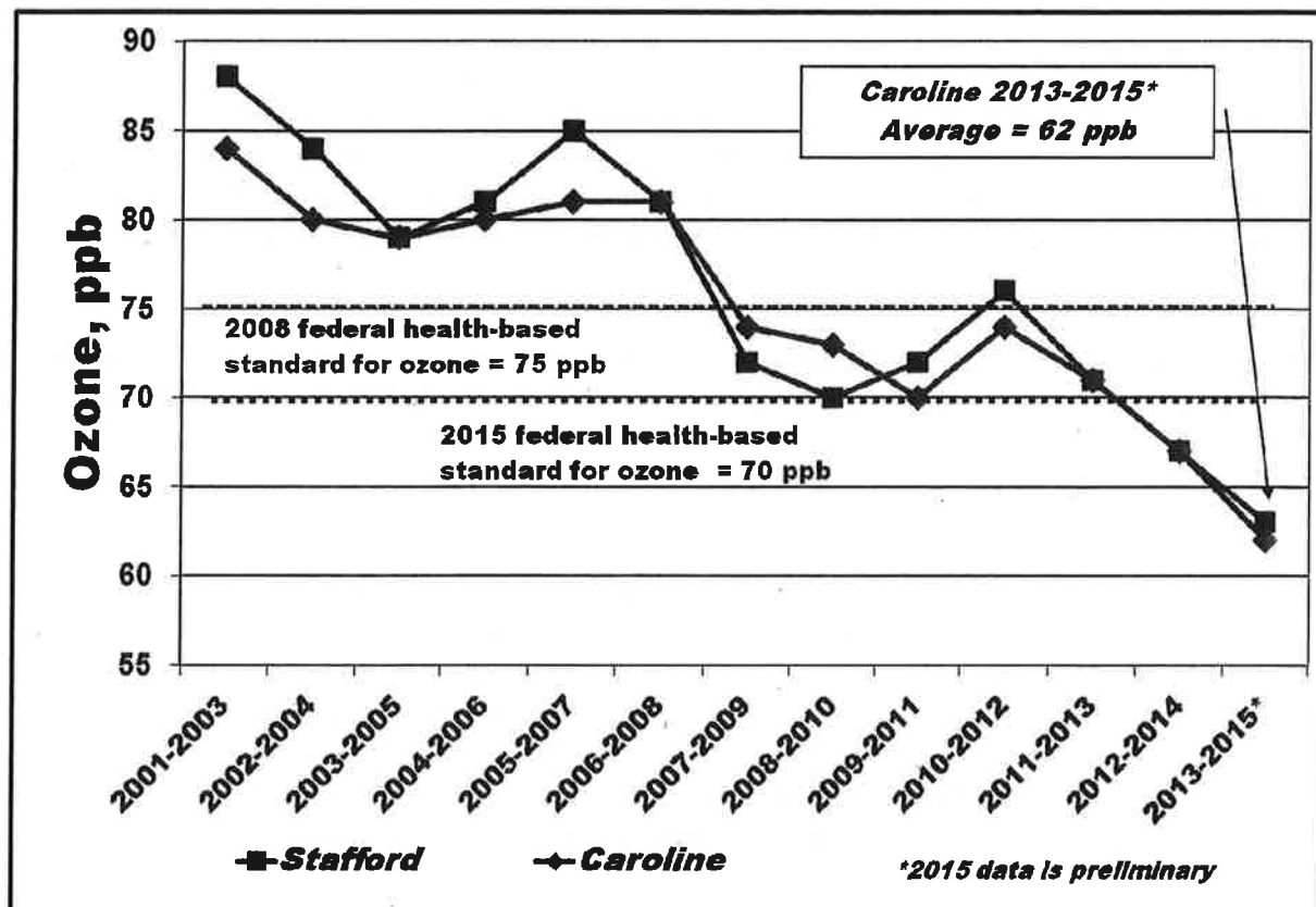
Figure 1: Ozone Air Quality, Caroline County and Stafford County
