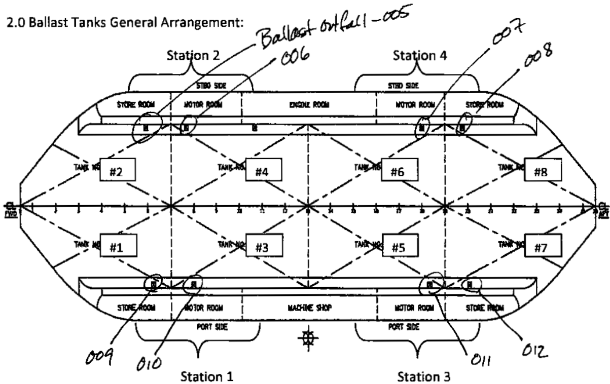
Figure = AFDL 21 General Arrangement of Ballast Tanks
