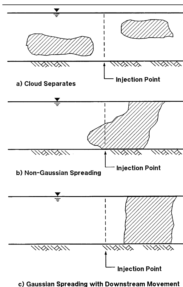
Figure 3-3. Vertical dye concentration profiles.
