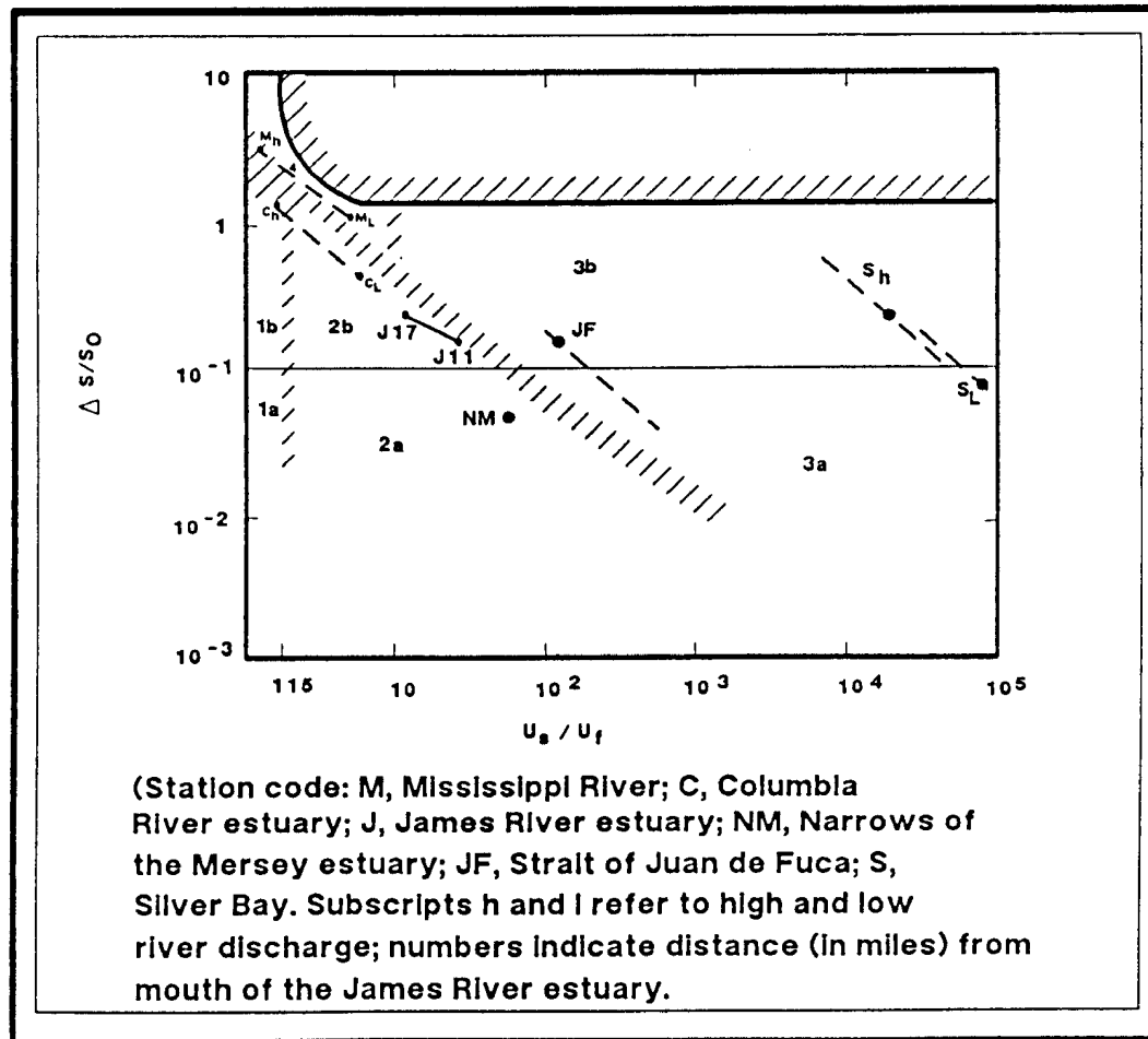
Figure 3-1. Stratification circulation diagram and examples.
