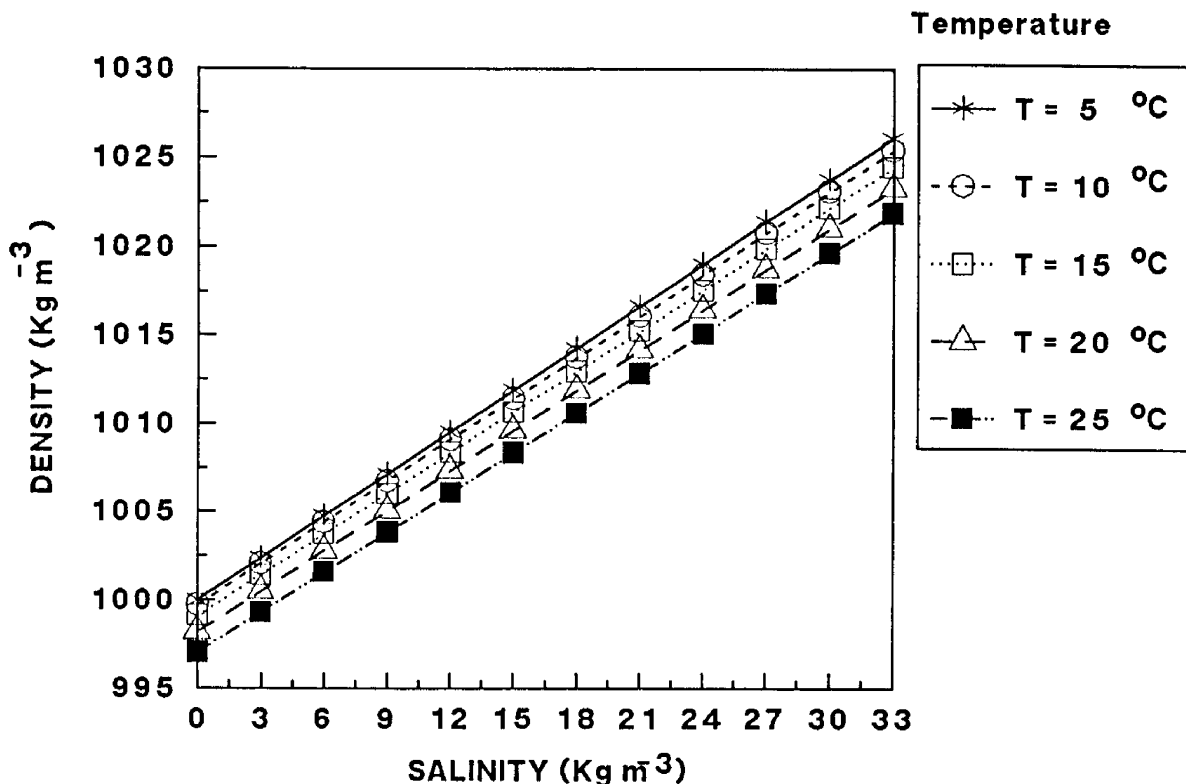
Figure 2-2. Relationship between water density, salinity, and temperature.
