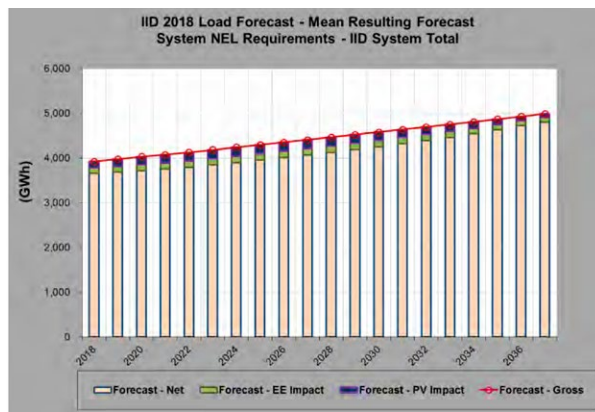
Figure 13. Imperial Irrigation District 2018 load forecast. Source: Imperial Irrigation District, www.iid.com/Home/ShowDocument?id=17371 .
