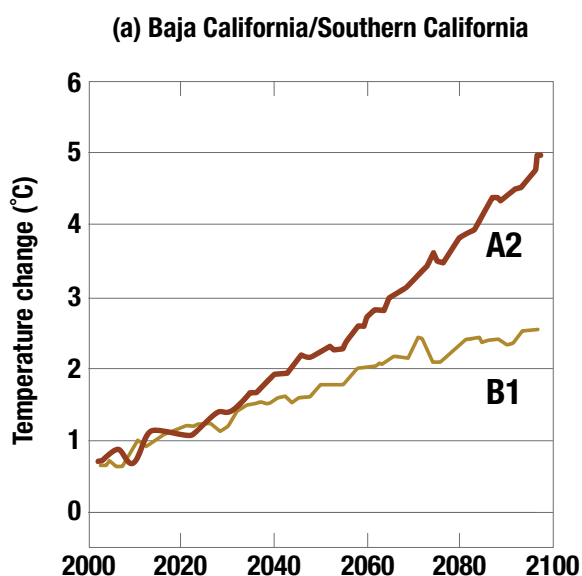
Figure 16. High- and low-emissions scenarios. A2: High-emissions scenario, B1: Low-emissions scenario.
