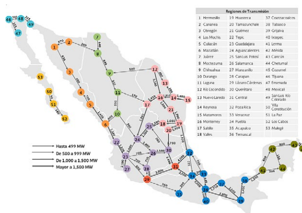
Figure 29. Capacity of the interconnections in the 53 regions of the National Electric System.
