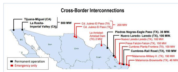
Figure 24. Cross-border interconnections.
