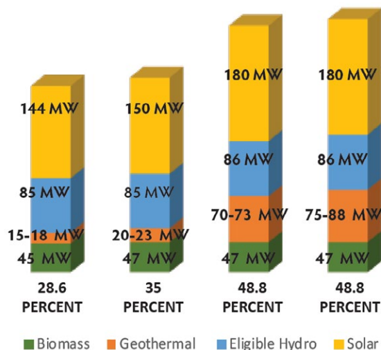
Figure 14. Actual/anticipated 2017–2020 renewables mix.
