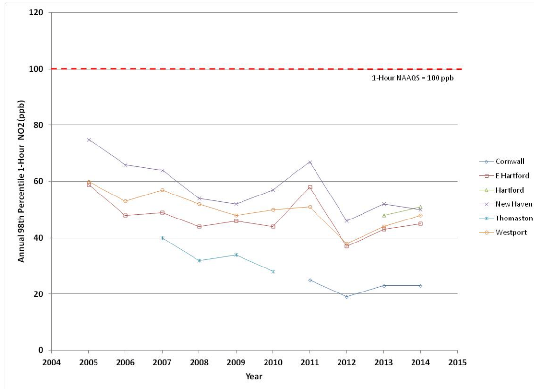
Figure 10: Connecticut 1-Hour † NO 2 Trends
