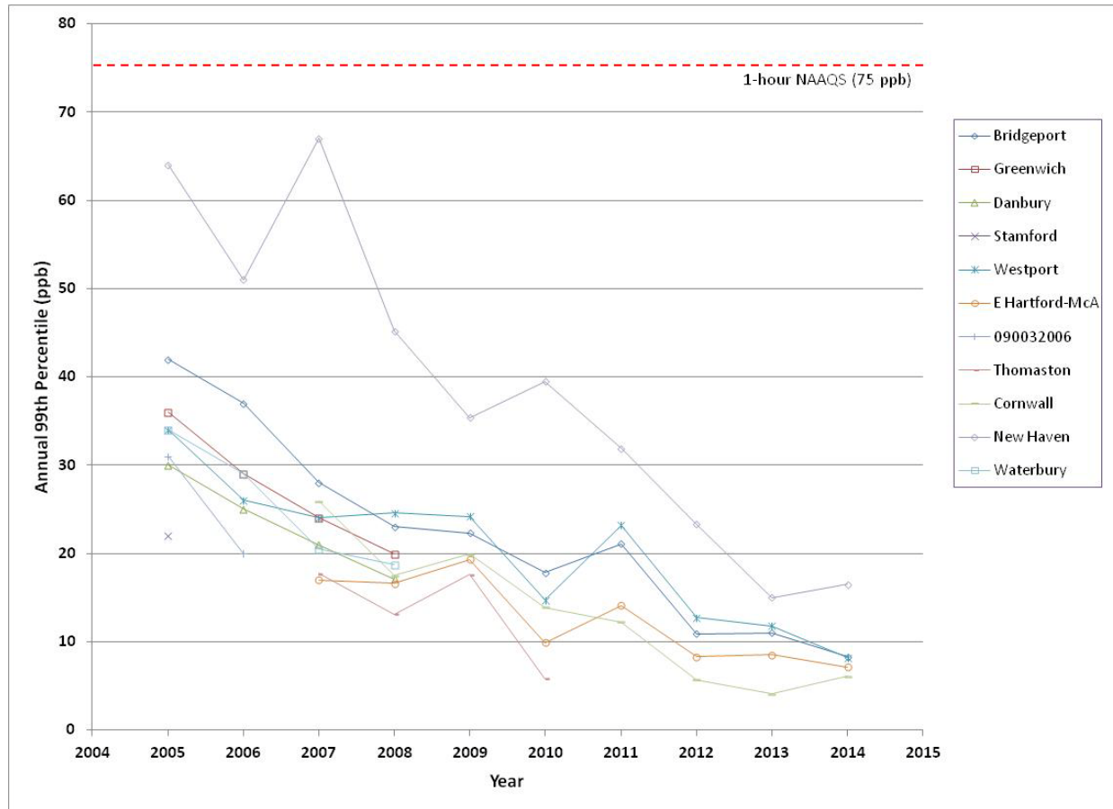
Figure 12: Connecticut Annual 99th Percentile Daily Maximum 1-hour SO 2 Values, 2005-2014
