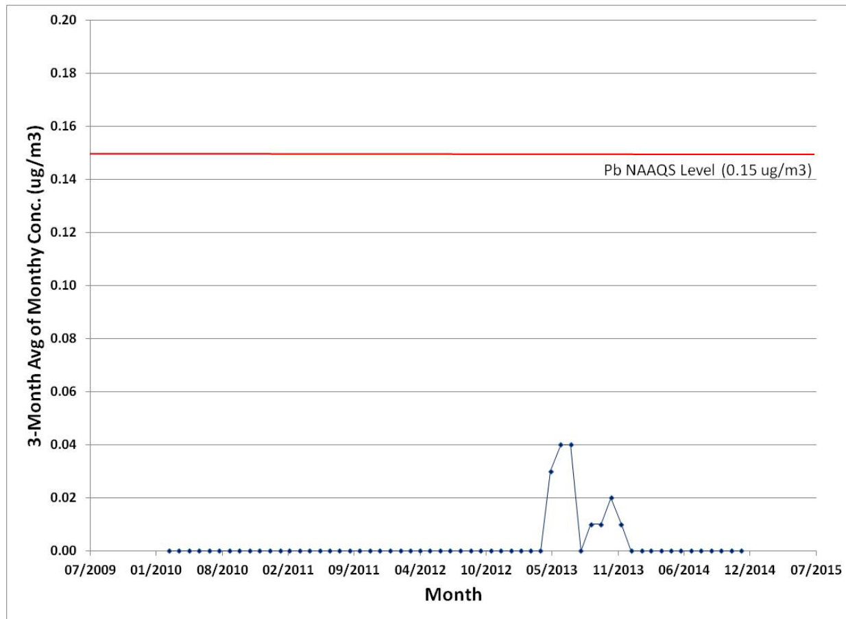
Figure 15: Pb-PM 10 Monitored Levels, 2010-2014
