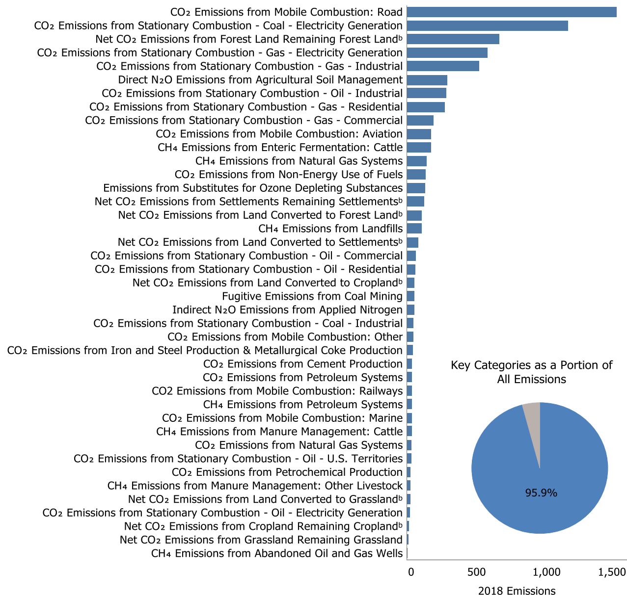
Figure ES-17: 2018 Key Categories (MMT CO 2 Eq.) a
