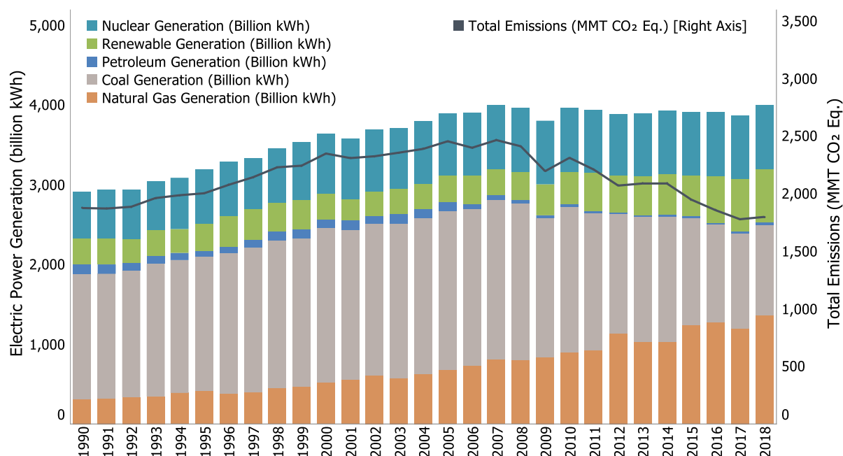
Figure ES-8: Electric Power Generation (Billion kWh) and Emissions (MMT CO 2 Eq.)
