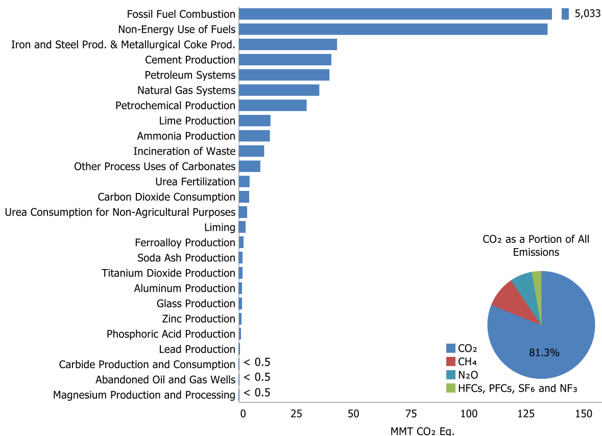
Figure ES-5: 2018 Sources of CO 2 Emissions (MMT CO 2 Eq.)
