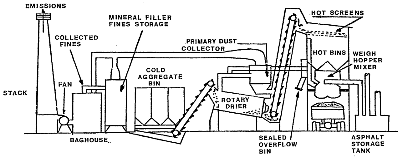
FIGURE 2: CONTROLLED HOT-MIX ASPHALT CONCRETE PLANT. (FROM REFERENCE 1)
