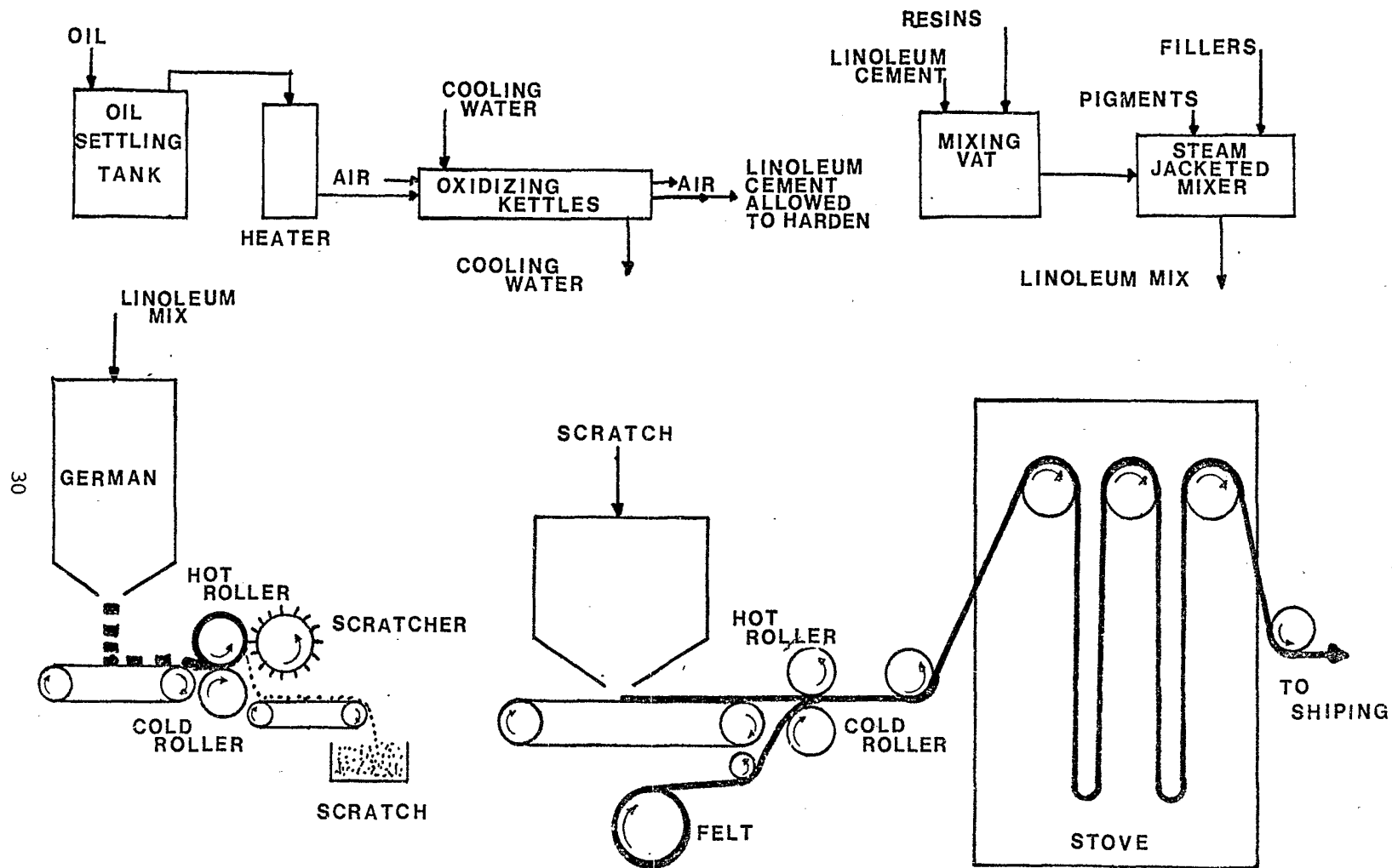
FIGURE 4 SCHEMATIC DRAWING OF LINE FOR MANUFACTURING LINOLEUM
