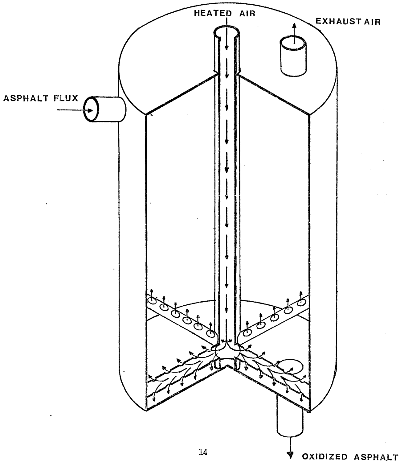
FIGURE 1 HALF SECTION VIEW OF ASPHALT OXIDIZING TOWER
