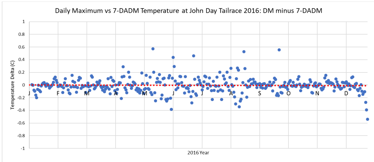
Figure 3: Delta between DM and 7-DADM (DM minus 7-DADM) at John Day Dam on the Columbia River for the year 2016. Trendline in red.
