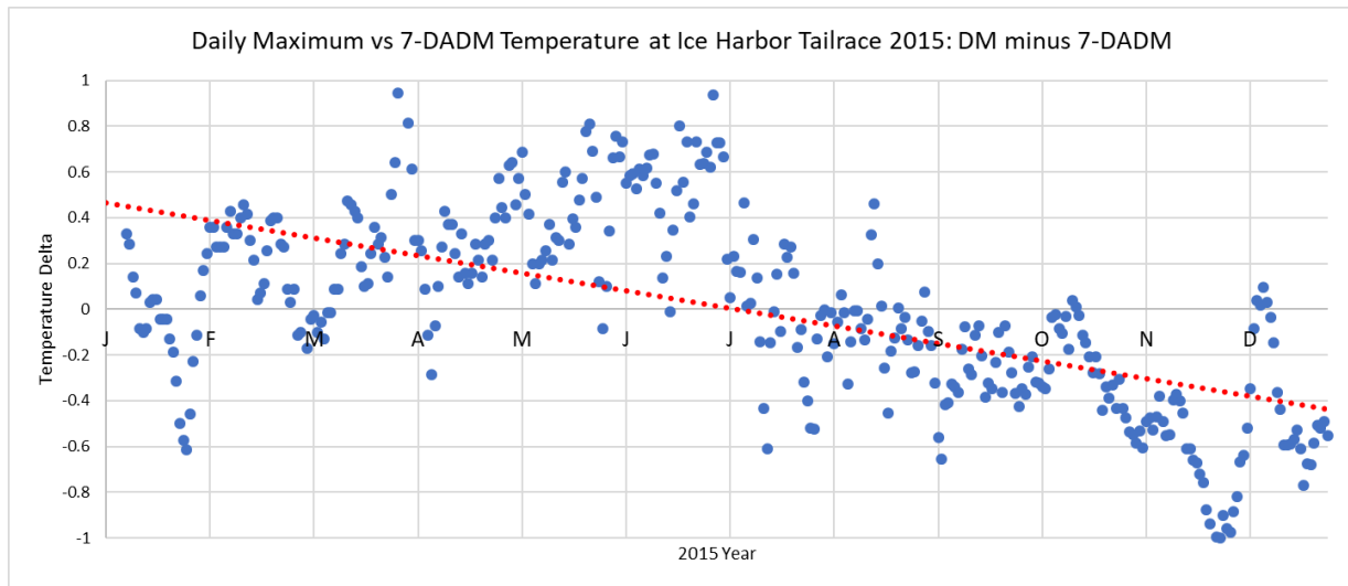
Figure 4: Delta between DM and 7-DADM (DM minus 7-DADM) at Ice Harbor Dam on the Snake River for the year 2015. Trendline in red.
