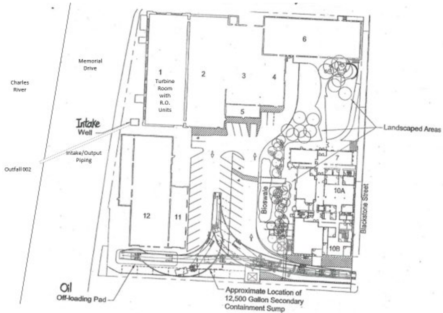
Figure 2: Site Plan
