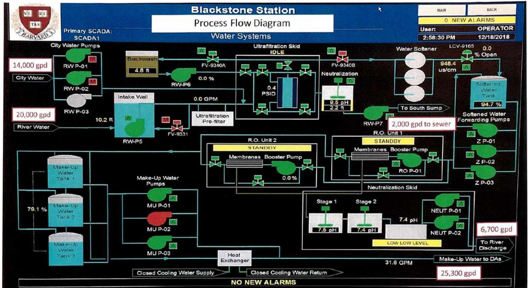
Figure 3: Schematic of Water Flow
