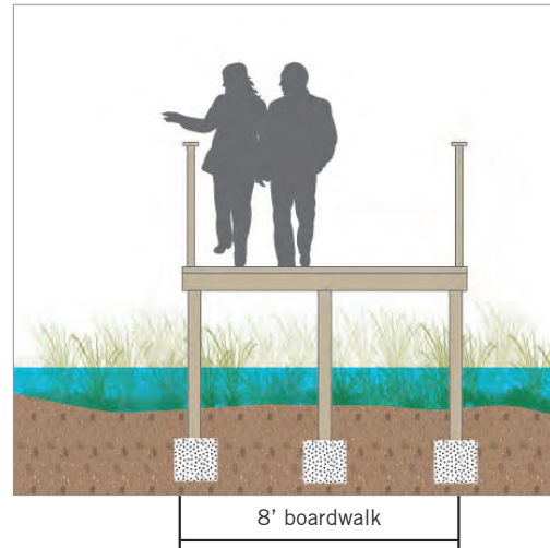
Section elevation of an 8' wide boardwalk in an area where flooding may occur frequently. Boardwalks with an elevation over 30" from ground require hand rails.
