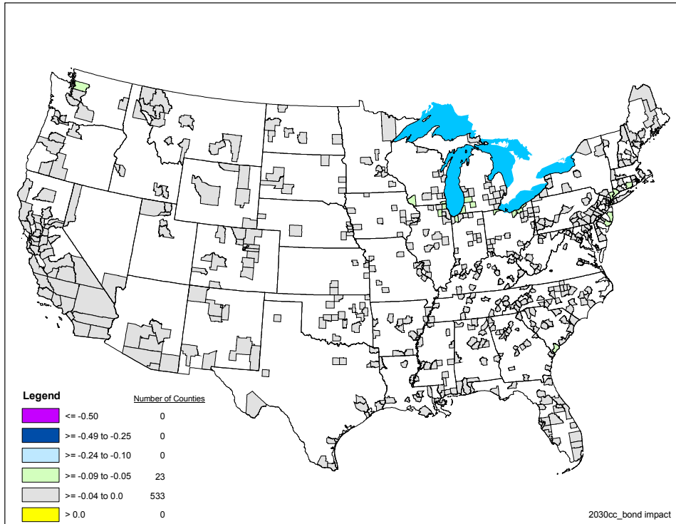
Figure III-7. Model-projected change in annual PM 2.5 design values from the small SI and marine SI control scenario in 2030. Units are \mu\text{g}/\text{m}^3 .
