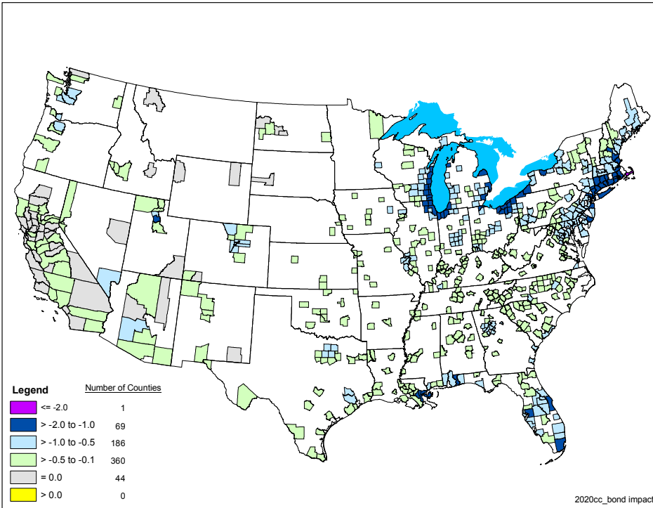
Figure III-1. Model-projected change in annual 8-hour ozone design values from the small SI and marine SI control scenario in 2020. Units are ppb.
