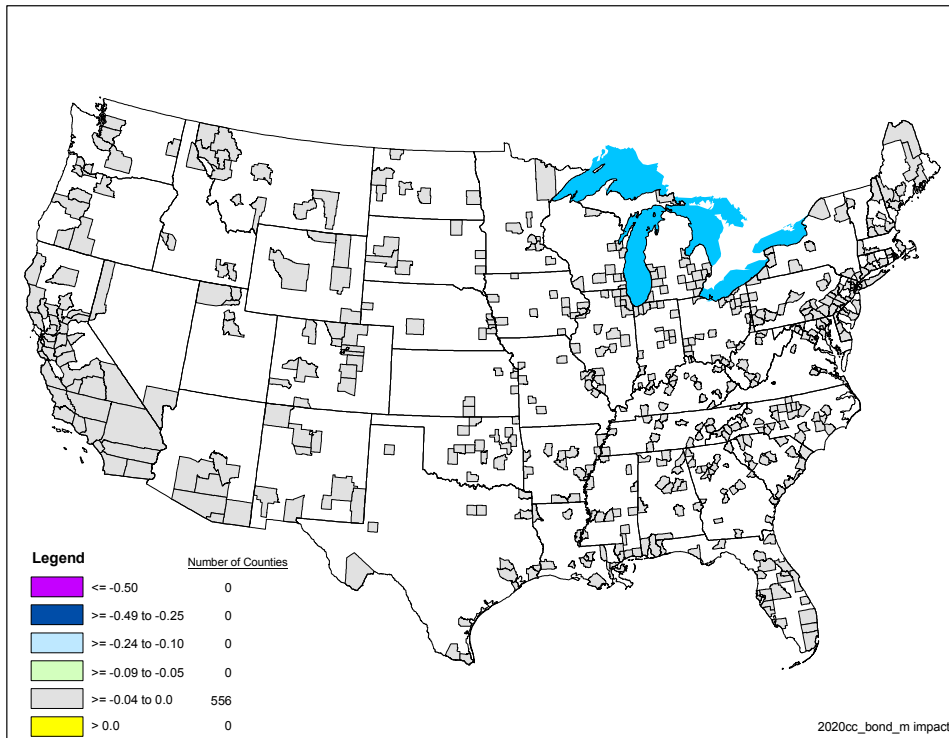
Figure III-6. Model-projected change in annual PM 2.5 design values from the marine SI control scenario in 2020. Units are \mu\text{g}/\text{m}^3 .
