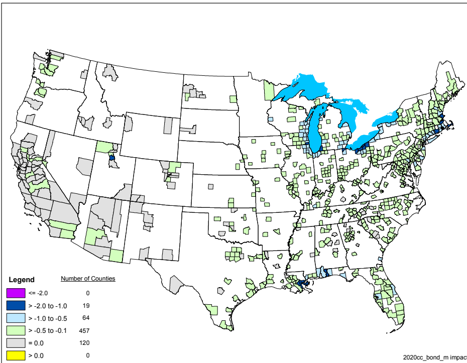
Figure III-2. Model-projected change in annual 8-hour ozone design values from the marine SI control scenario in 2020. Units are ppb.
