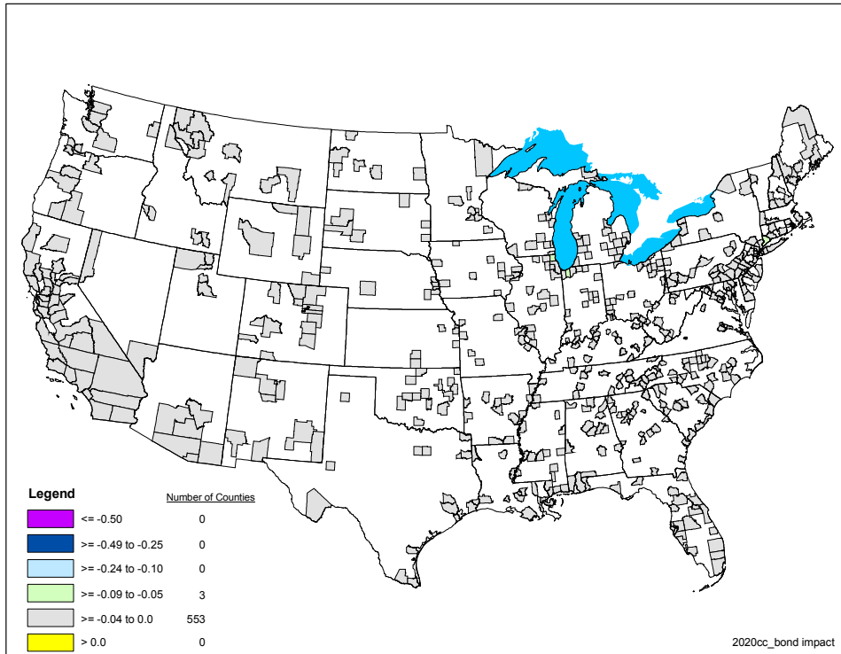
Figure III-5. Model-projected change in annual PM 2.5 design values from the small SI and marine SI control scenario in 2020. Units are \mu\text{g}/\text{m}^3 .
