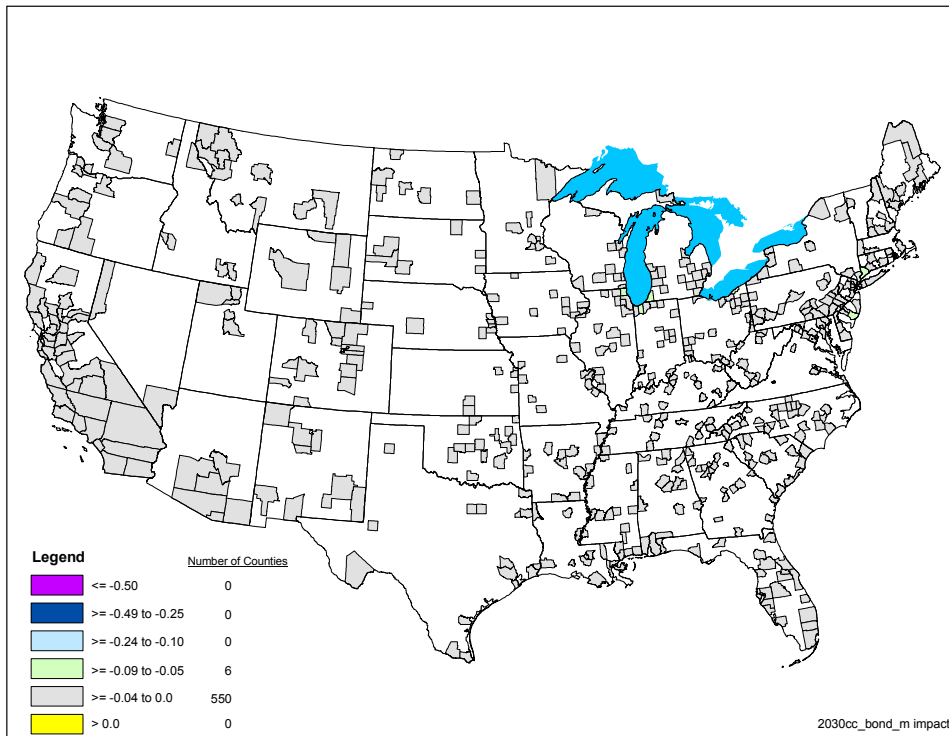
Figure III-8. Model-projected change in annual PM 2.5 design values from the marine SI control scenario in 2030. Units are \mu\text{g}/\text{m}^3 .
