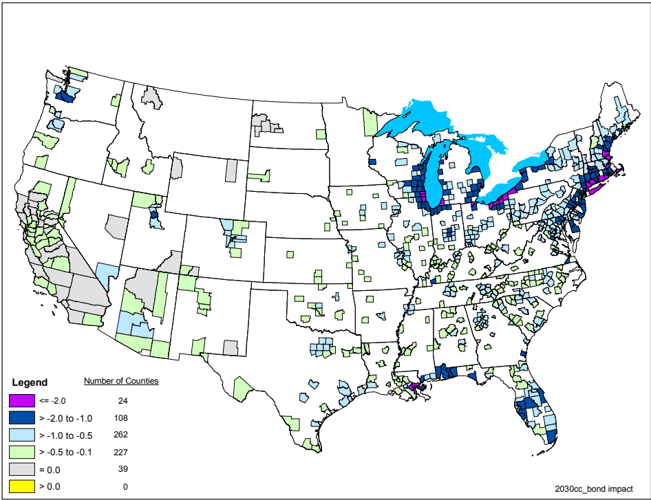
Figure III-3. Model-projected change in annual 8-hour ozone design values from the small SI and marine SI control scenario in 2030. Units are ppb.
