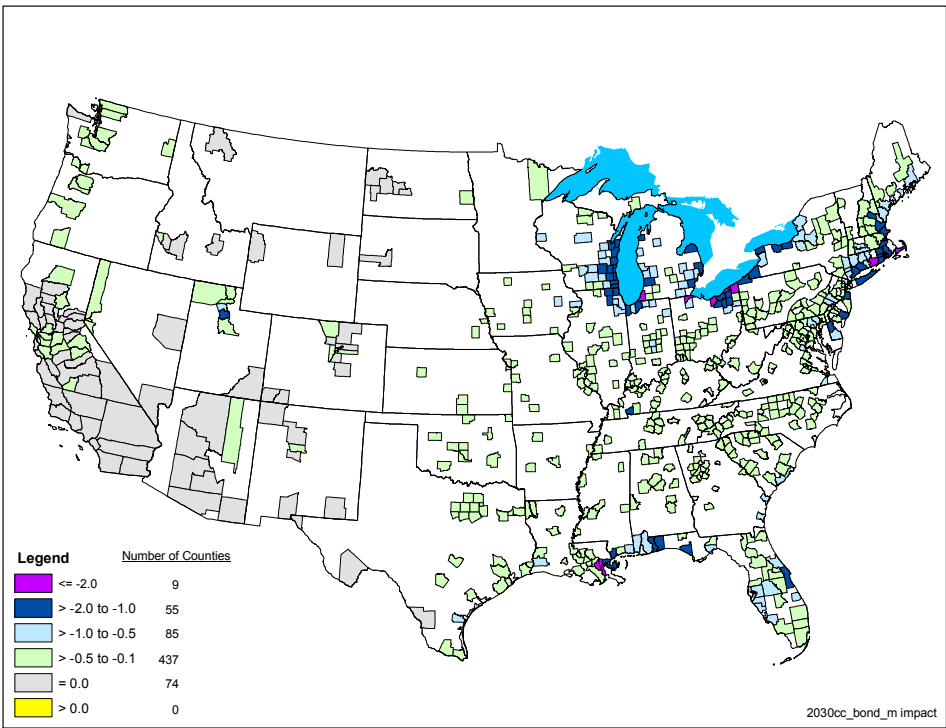
Figure III-4. Model-projected change in annual 8-hour ozone design values from the marine SI control scenario in 2030. Units are ppb.
