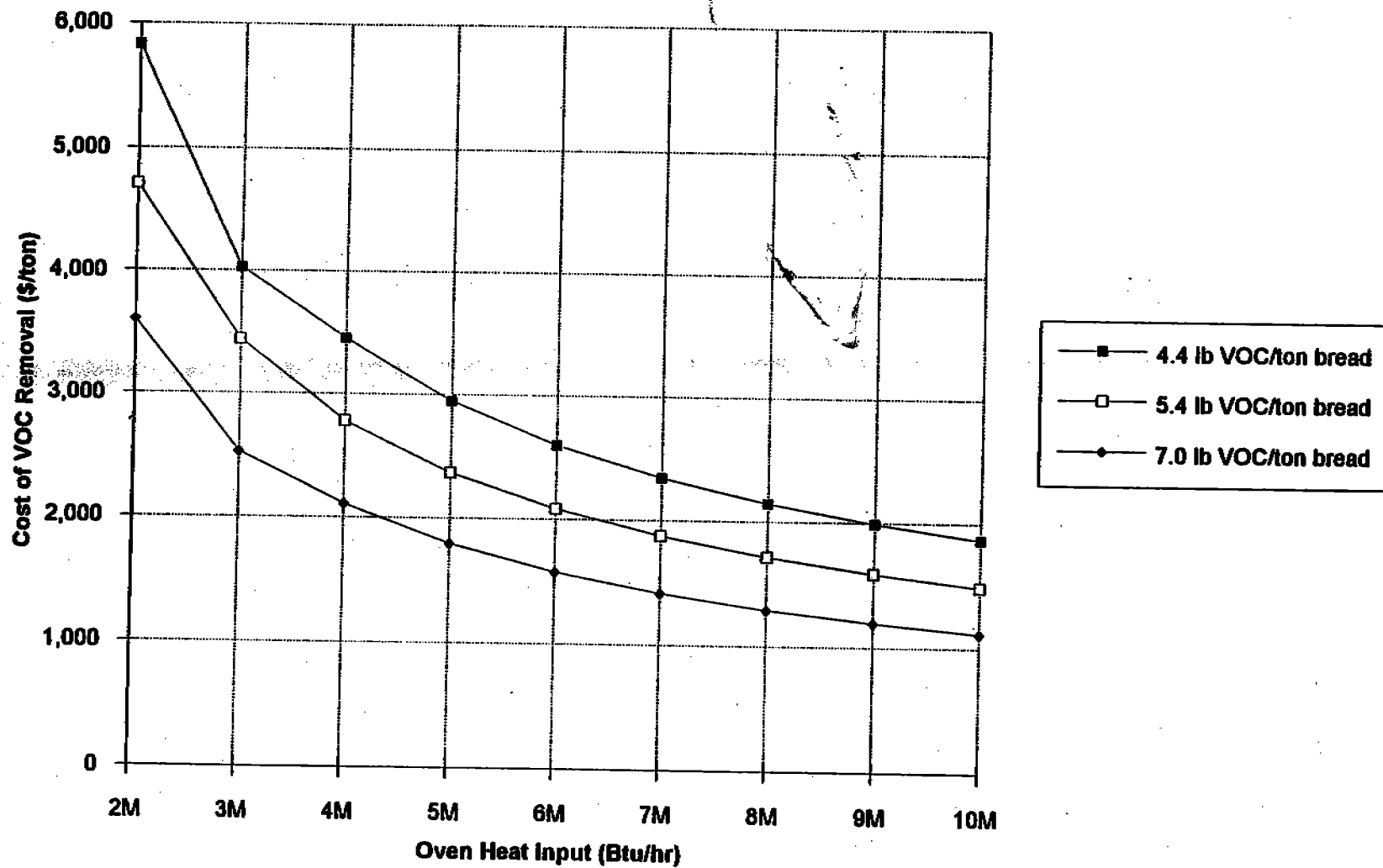
Figure 4-2 Cost Effectiveness of Regenerative Oxidation on Bakery Ovens
