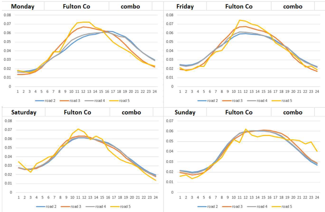
Figure 3-20. Example of Temporal Profiles for Combination Trucks
