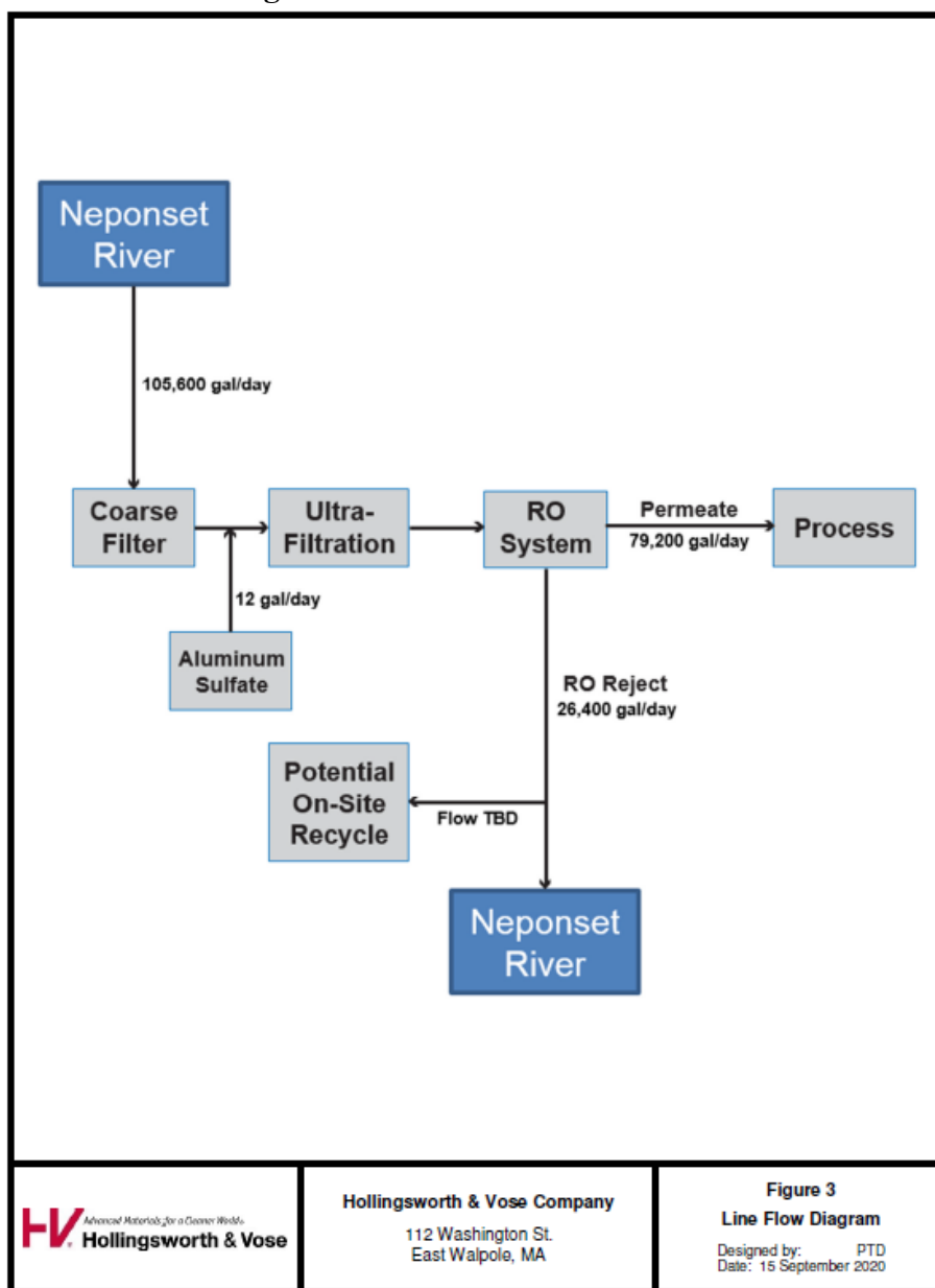
Figure 3: Schematic of Water Flow
