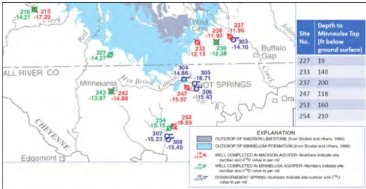
Figure Q. Locations of springs emanating from or passing through the Minneulsa aquifer, from Figure 8 of Naus et al., 2001.
