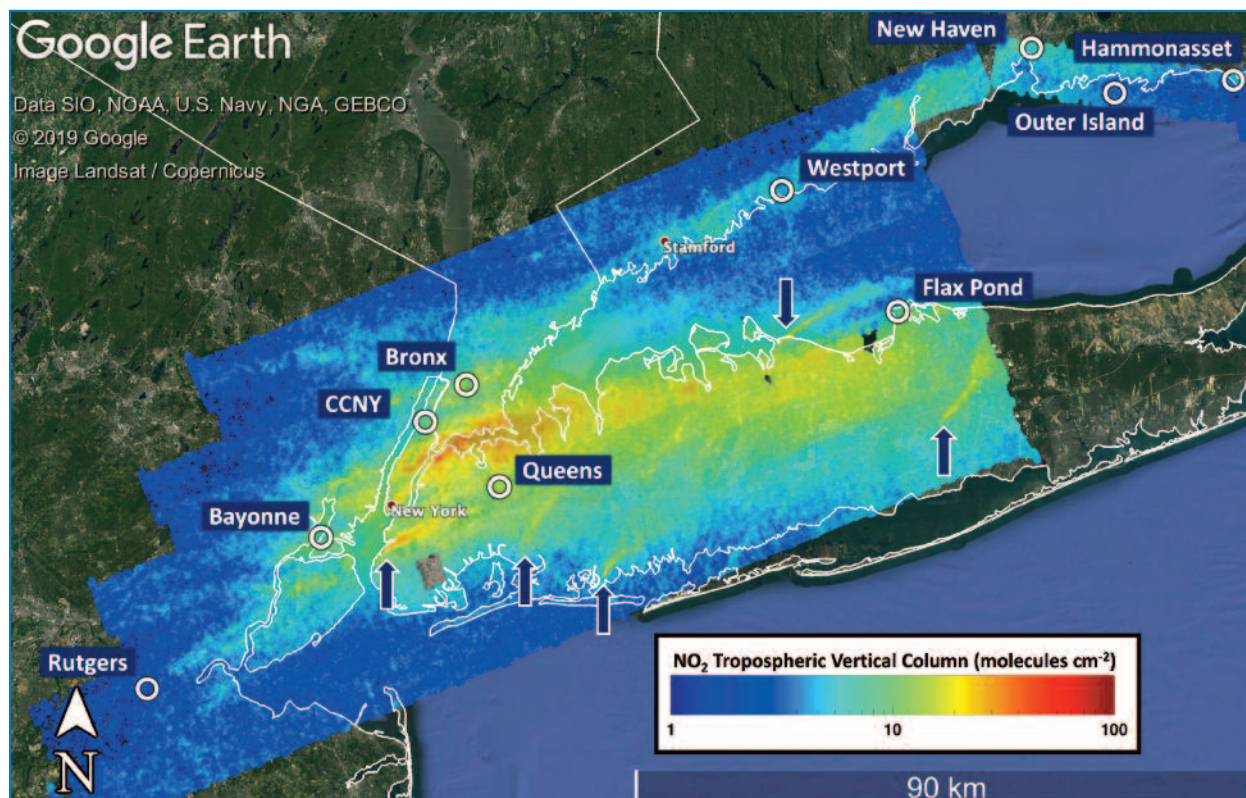
Figure 4. NASA aircraft measurements (GCAS) of tropospheric NO 2 columns on August 28, 2018, observed between 1:00 pm and 4:00 pm EDT. Circles indicate ground monitoring sites. Arrows point to sources of visible pollution plumes.
