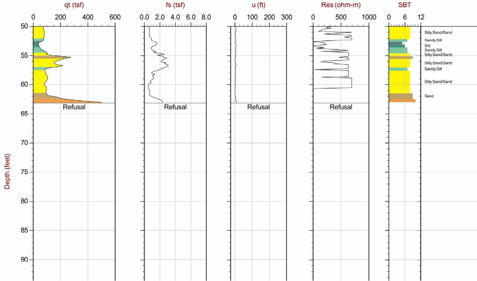
Figure B5. CPT for Boring B10 (continued)
