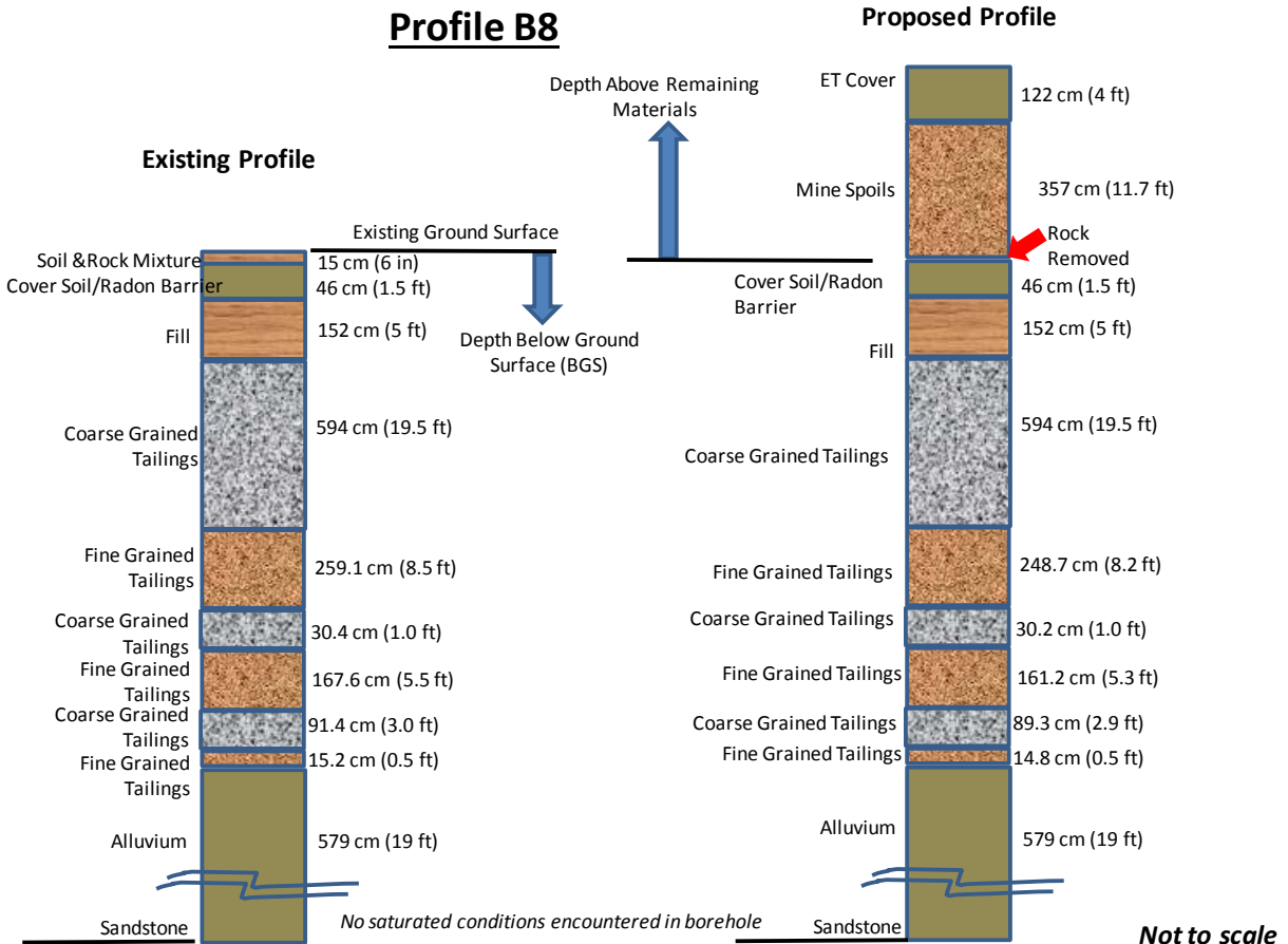
Figure 9. Profile B8
