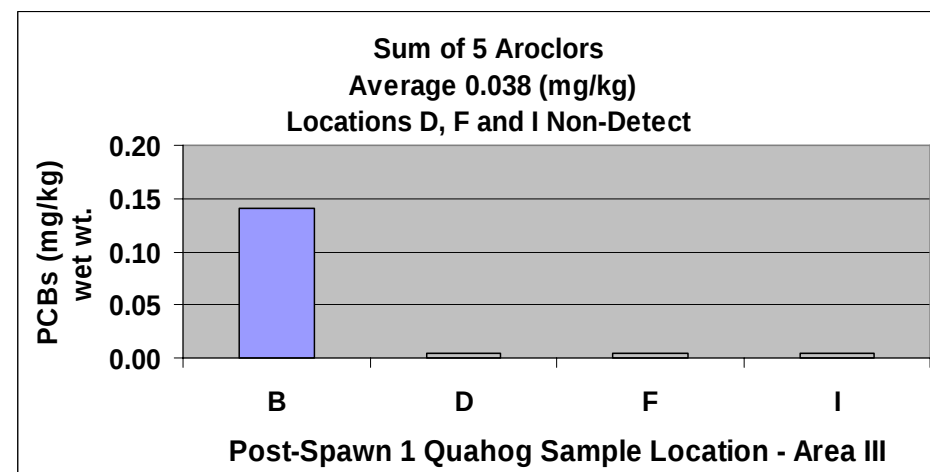
Figure 8 PCBs Concentrations in Post-Spawn 1 Quahog 2008
