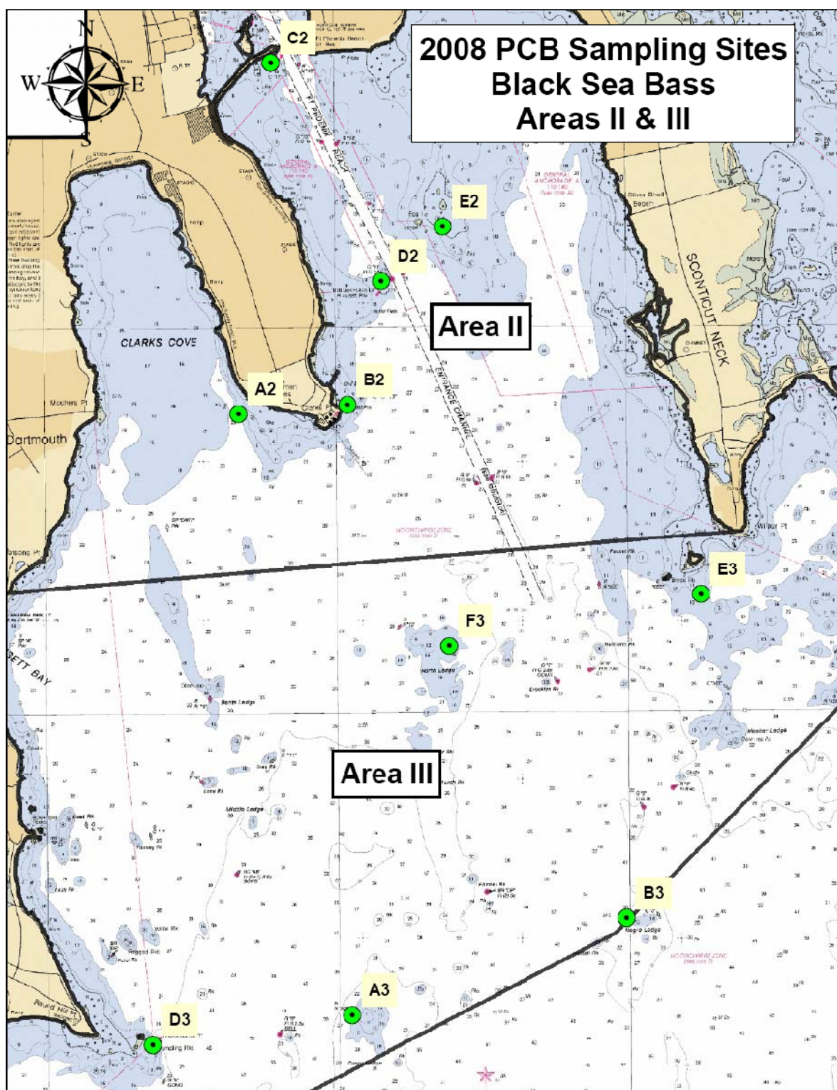
Figure 3 Sea Bass Sample Locations - Area II & III
