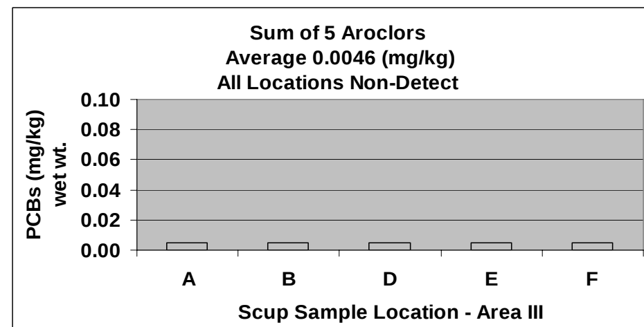
Figure 11 PCBs Concentrations in Scup 2008
