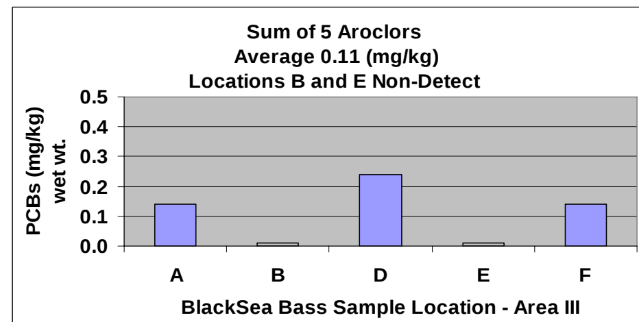
Figure 10 PCBs Concentrations in Black Sea Bass 2008
