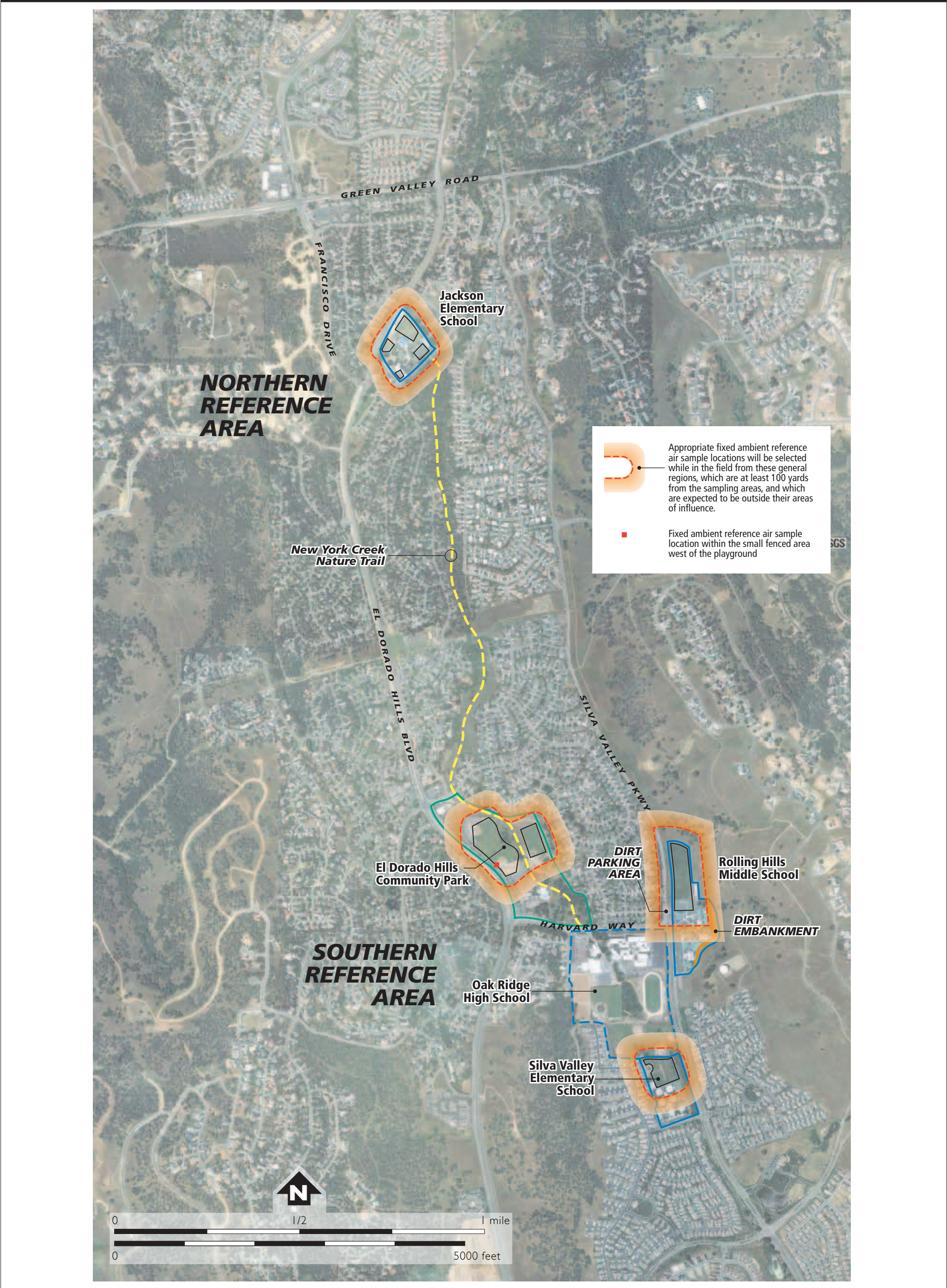
Figure 2-2 Fixed Ambient Reference Air Sampling Location Map
