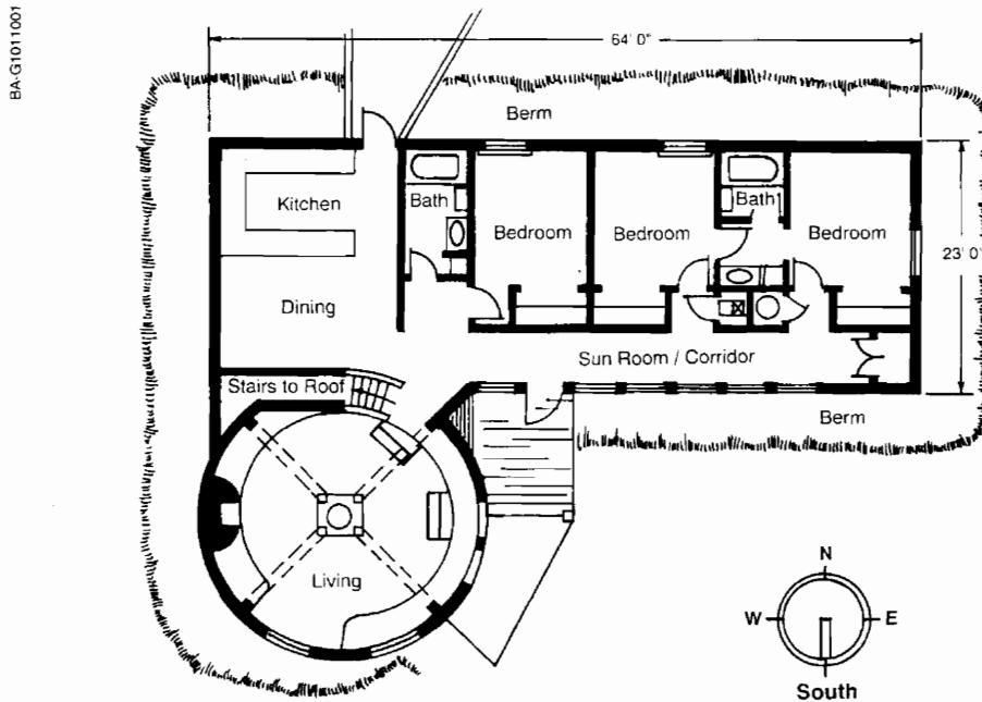
Floor Plan
