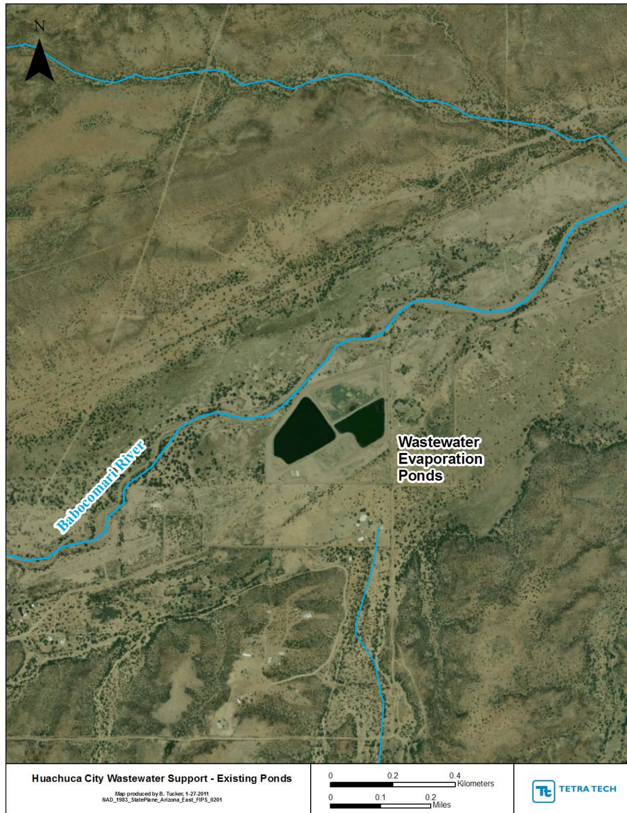
Figure 2. Aerial Image of Existing Wastewater Ponds
